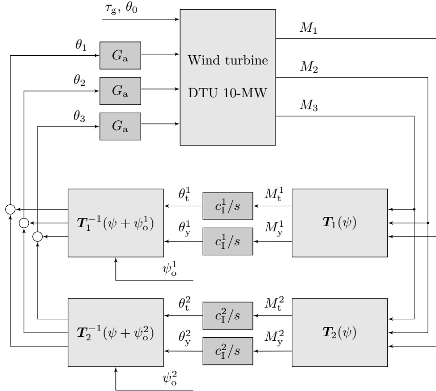
Figure 1: Implementation of IPC using the azimuth-dependent forward and reverse transformations, T_n(\psi) and T_n^{-1}(\psi + \psi_o^n) , respectively. The transformations are used to form two feedback loops at the 1P and 2P rotational frequencies, transforming the blade load harmonics to a fixed reference frame. For both 1P and 2P loops in the fixed frame, the tilt- and yaw-axis loads signals are subject to integral action using equal gains for both axes. After the reverse transformation – including separate azimuth offsets \psi_o^n – the 1P and 2P contributions are summed to form the implementable IPC signals \theta_i for attenuation of the respective blade out-of-plane harmonic loads. A pitch actuator model G_a is included. The collective pitch and generator torque control signals, \theta_0 and \tau_g , are generated by turbine controllers, which are omitted in this figure.
