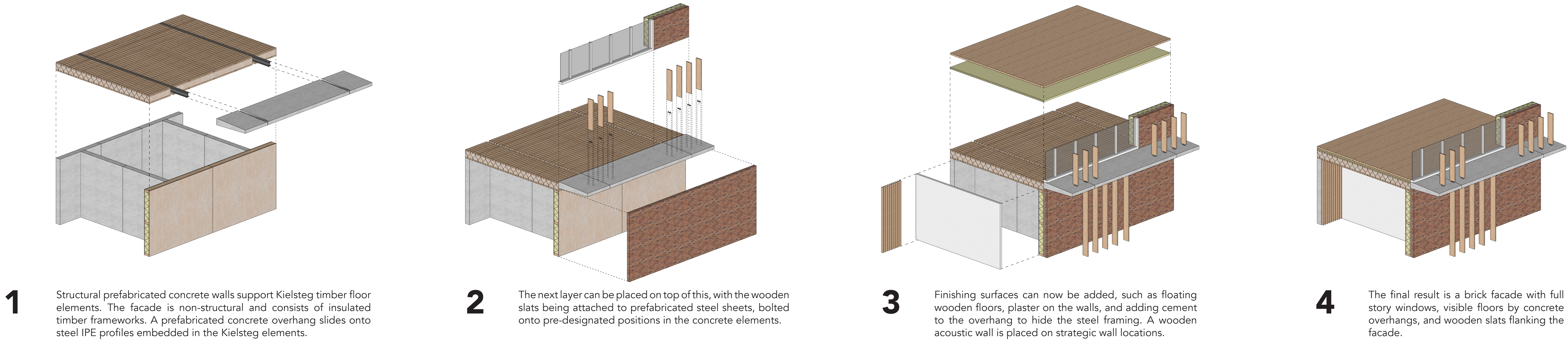
SCHEMATIC ASSEMBLY PROCESS OVERVIEW
