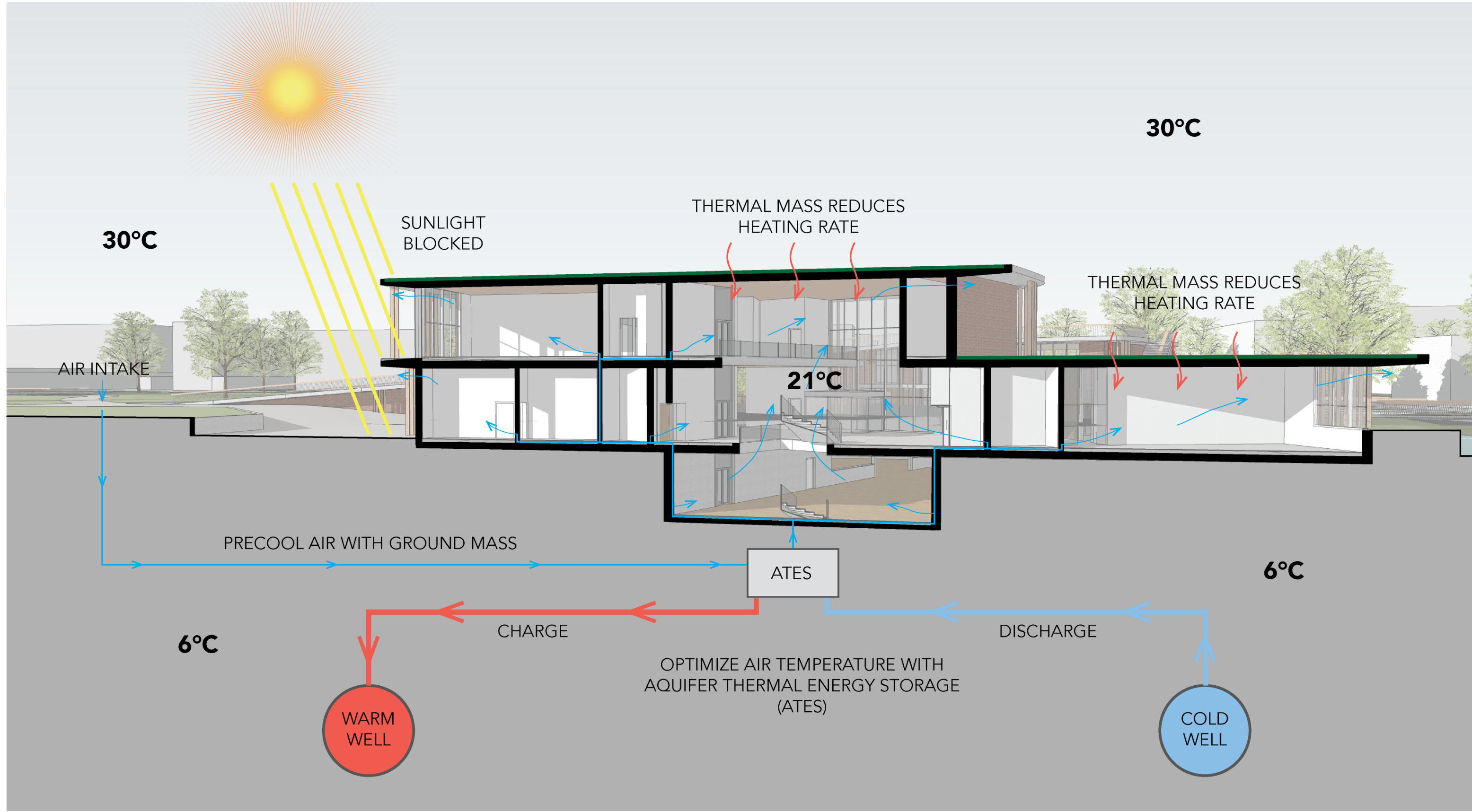
SUMMER CLIMATE DIAGRAM
