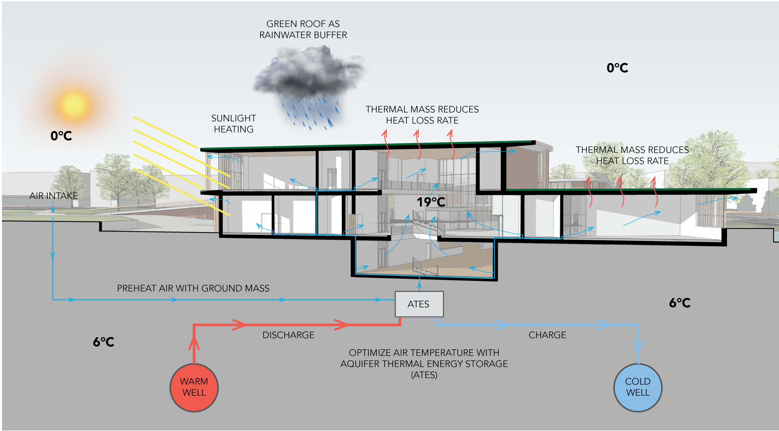
WINTER CLIMATE DIAGRAM
