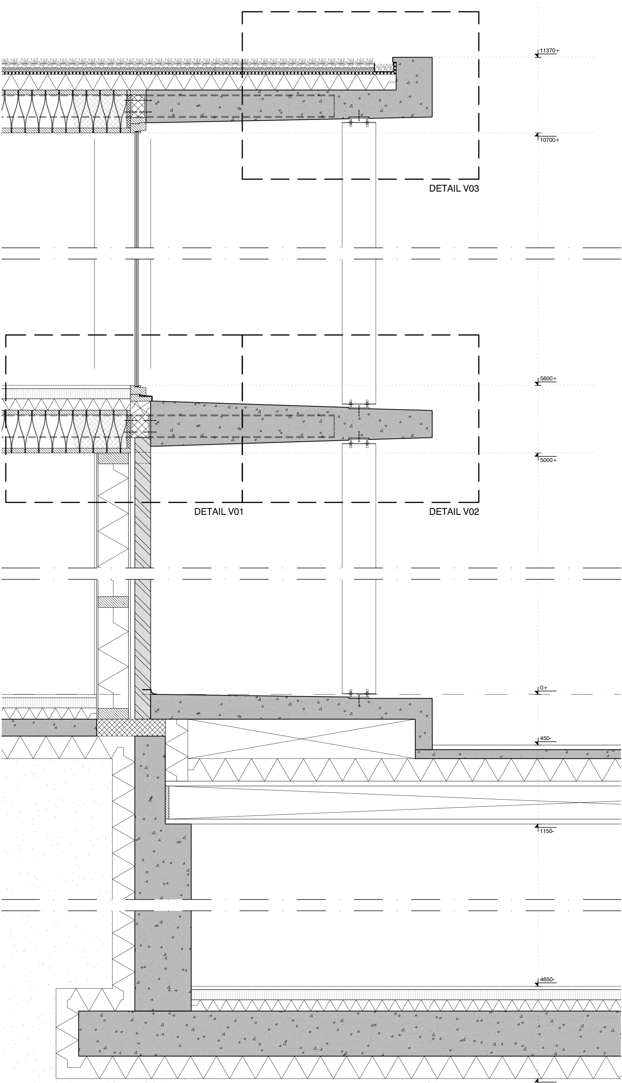
CROSS SECTION
