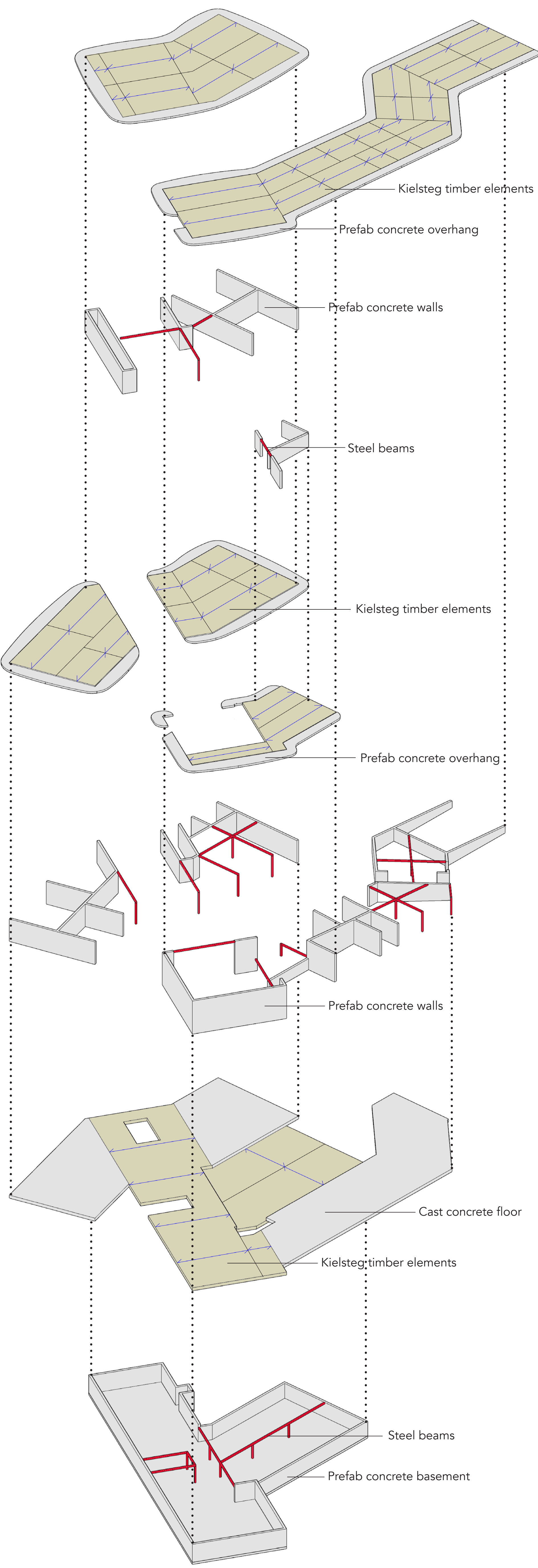
EXPLODED AXONOMETRIC STRUCTURE OVERVIEW
