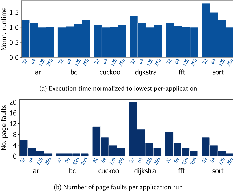
Fig. 12. Effect of page size (in bytes).
