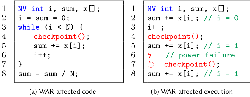
Fig. 2. WAR dependency example. NV marks non-volatile variables, checkpoint() is a checkpoint of volatile state.
