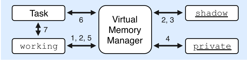
Fig. 7. Interaction among task, memory manager, and memory buffers upon RP and WP and order of occurrence. Steps 2, 3, 4, and 5 are conditional.
