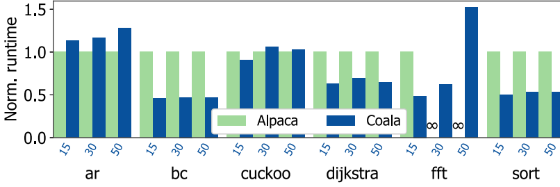
Fig. 11. Coala’s execution time normalized to Alpaca’s, for three distances from the energy source (15, 30, and 50 cm).
