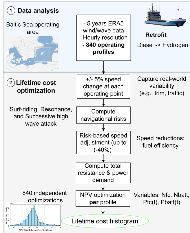
Figure 5.2: Methodology diagram
