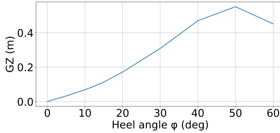
Figure 4.9: GZ curve
