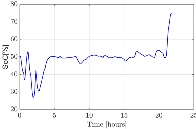
Figure 3.5: Constant power profile — battery SoC.
