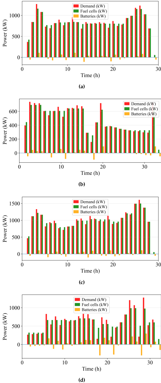
Figure 5.8: Vessel power profiles for different weather conditions: (a) Average-power, (b) Low-power, (c) High-power, (d) Fluctuating (short-period high peak).
