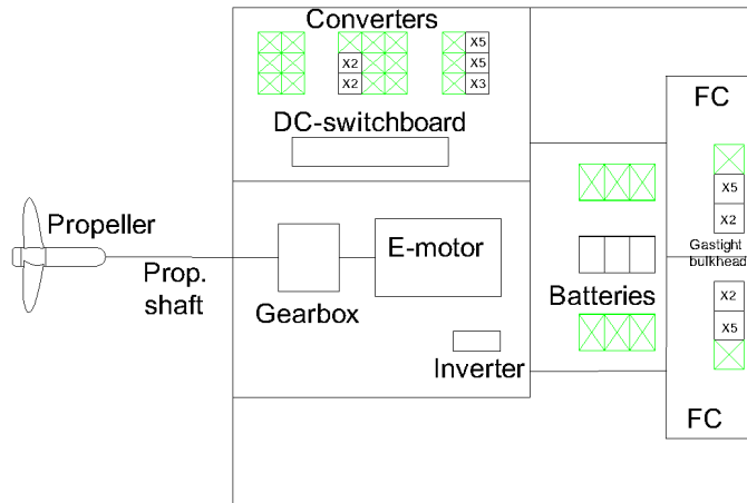
Figure 4.4: Engine room layout for the optimal propulsion system design
