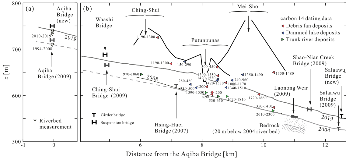
Fig. 6. Engineered structures and dated deposits along a segment of the Laonong river valley, shown relative to long river profiles and to truncated debris fans. A date in parentheses indicates the year of destruction of a structure. Dated sample: Debris fan deposits (red triangle), dammed lake deposits (blue triangle), and trunk river deposits (green triangle).
