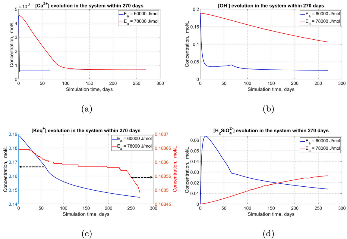
Fig. 9. Comparison of the ion concentration evolution between system A and system B within 270 days. (a): The change of [Ca^{2+}] ; (b): The change of [OH^-] ; (c): The change of [K_{eq}^+] ; (d): The change of [H_2SiO_4^{2-}] ; The concentration of each ion is the total moles of each ion divided by the total volume of the domain, which is 1 \times 10^{-12} m^3 .
