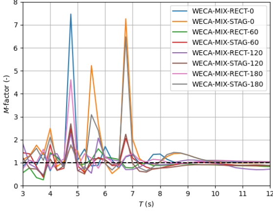
Fig. 15. M -factor for PA and flap mixed farms in regular waves
