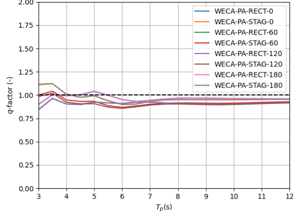
Fig. 16. q -factor for PA mono-farms in irregular waves ( H_s = 1 m)
