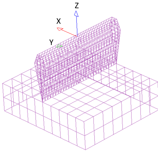
Fig. 2. Mesh of flap modelled using HAMS-MREL
