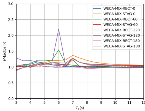
Fig. 19. H -factor for PA and flap mixed farms in irregular waves ( H_s = 1 m)
