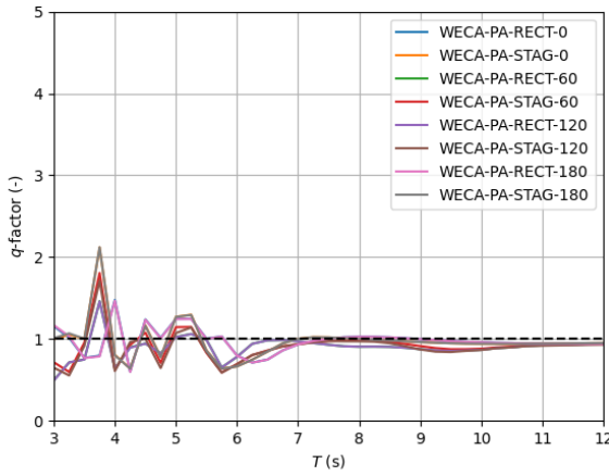
Fig. 11. q -factor for PA mono-farms in regular waves
