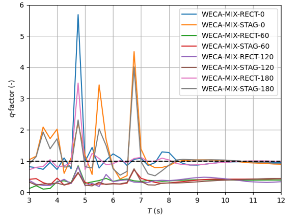
Fig. 13. q -factor for PA and flap mixed farms in regular waves
