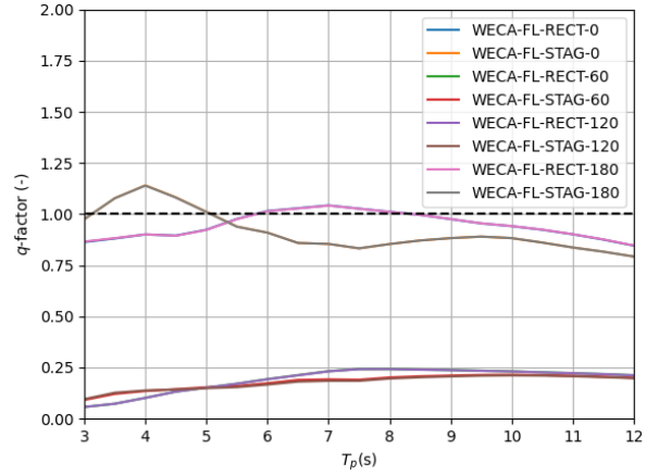
Fig. 17. q -factor for flap mono-farms in irregular waves ( H_s = 1 m)
