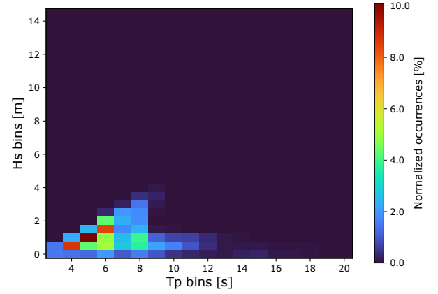
Fig. 10. Scatter diagram off the dutch coast(latitude: 53^\circ 36' , longitude: 6^\circ 18' )
