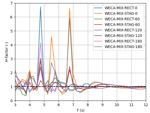
Fig. 14. H -factor for PA and flap mixed farms in regular waves
