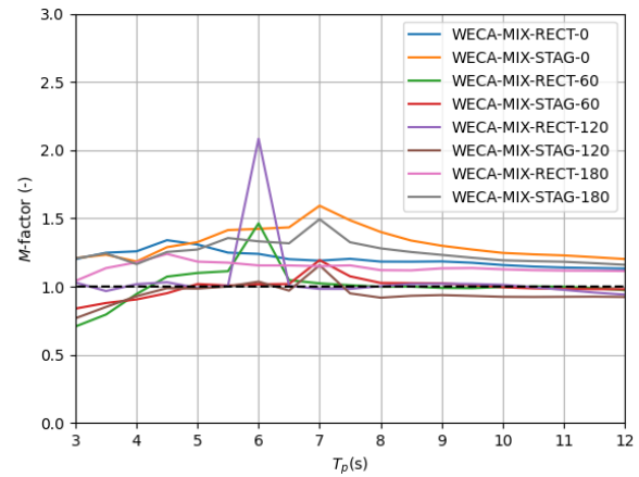
Fig. 20. M -factor for PA and flap mixed farms in irregular waves ( H_s = 1 m)
