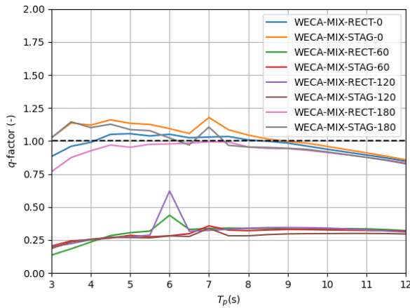
Fig. 18. q -factor for PA and flap mixed farms in irregular waves ( H_s = 1 m)
