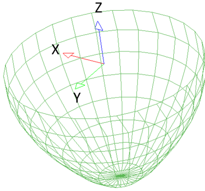
Fig. 1. Mesh of Point absorber modelled using HAMS-MREL
