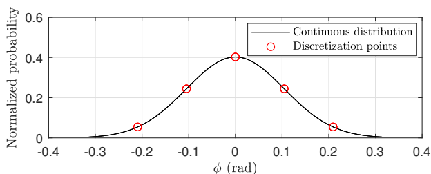
Fig. 11. Robust optimization
