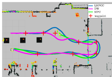
Fig. 7. Static collision avoidance scenario. The red crosses depict the path to follow (waypoints) and the colored points are the laser scan data. The blue, green, and magenta lines represent the trajectory obtained with the LMPPC, the MPC tracking controller, and the Dynamic Window, respectively.
