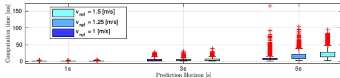
Fig. 6. Computation time required to solve the LMPPC problem online for different velocity references and horizon lengths. The central mark indicates the median. The bottom and top edges of the box indicate the 25th and 75th percentiles, respectively. The red crosses represent the outliers.
