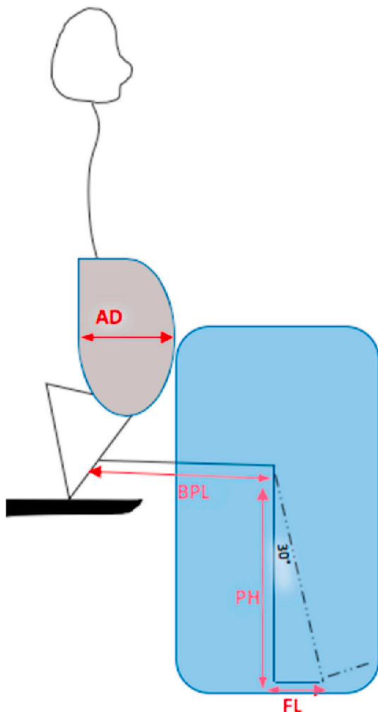
Fig. 3. Legroom depth equation considering abdominal depth.
