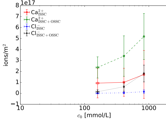
Figure 4.12: Ion surface density based on ion adsorption type.
