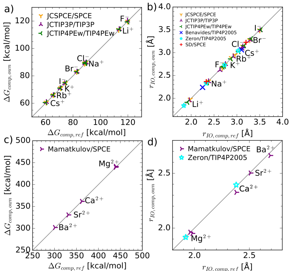
Figure 2.3: Verification of our methodology by reproducing the results from Smith and Dang [17], Benavides et al. [21], Joung and Cheatham [18] and Mamatkulov et al. [19]. (a) and (c) show the \Delta G_{solv} and (b) and (d) the r_{IO} .
