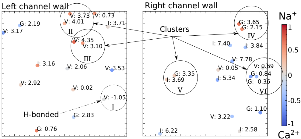
Figure 3.12: Preferential adsorption of \text{Na}^+ (red) and \text{Ca}^{2+} (blue) on dangling oxygens on the left and right surfaces of the channel. The letters indicate the type of silanol (i.e. Isolated, Vicinal and Geminal) and the number a protrusion metric times 100 given by equation 3.13. Regions I-VI are specifically discussed in the main text.
