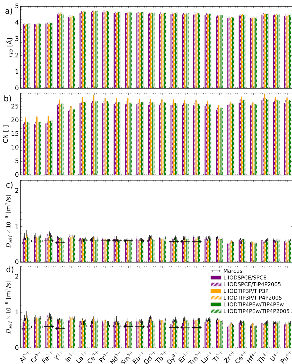
Figure 2.14: Radius (a) and coordination number (b). Scaled diffusion coefficients by \eta_{model}/\eta_{exp} (c) and by D_{i,exp}/D_{i,model} (d) for trivalent cations optimized for r_{10} .
