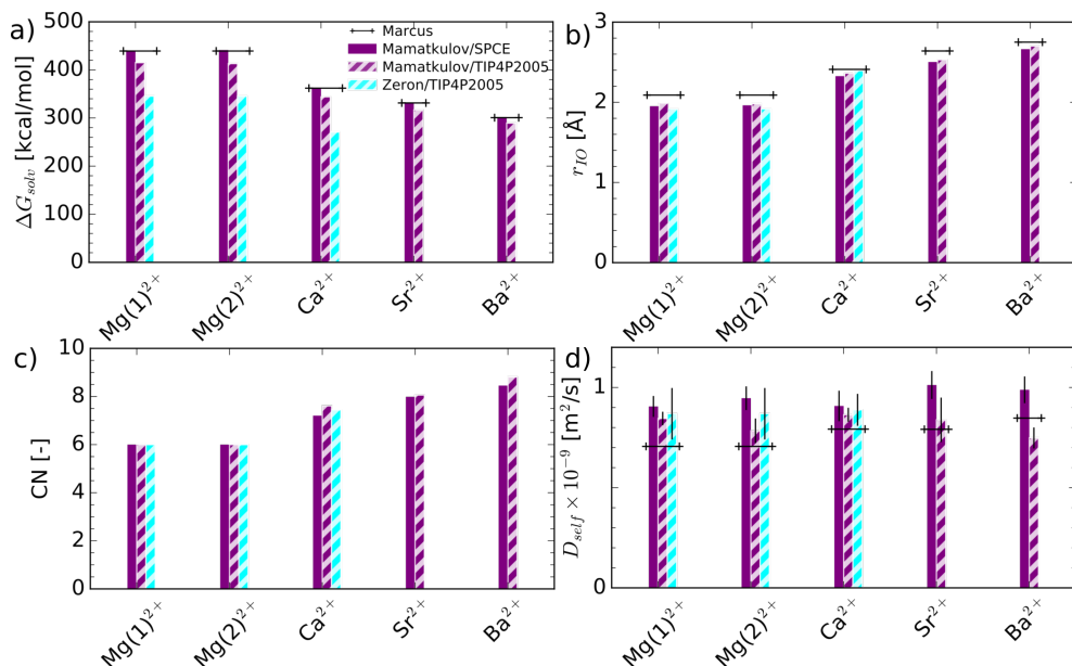
Figure 2.6: Transferability of divalent cation parameters in terms of \Delta G_{\text{solv}} (a), r_{10} (b), CN (c) and D_{i,\text{self}} (d). \text{Mg}^{2+}(1) and \text{Mg}^{2+}(2) account for both parametrizations of Mamatkulov et al. [19]. 95 % uncertainty is shown for D_{i,\text{self}} . Other uncertainties were negligible. Experimental results are from Marcus [97].
