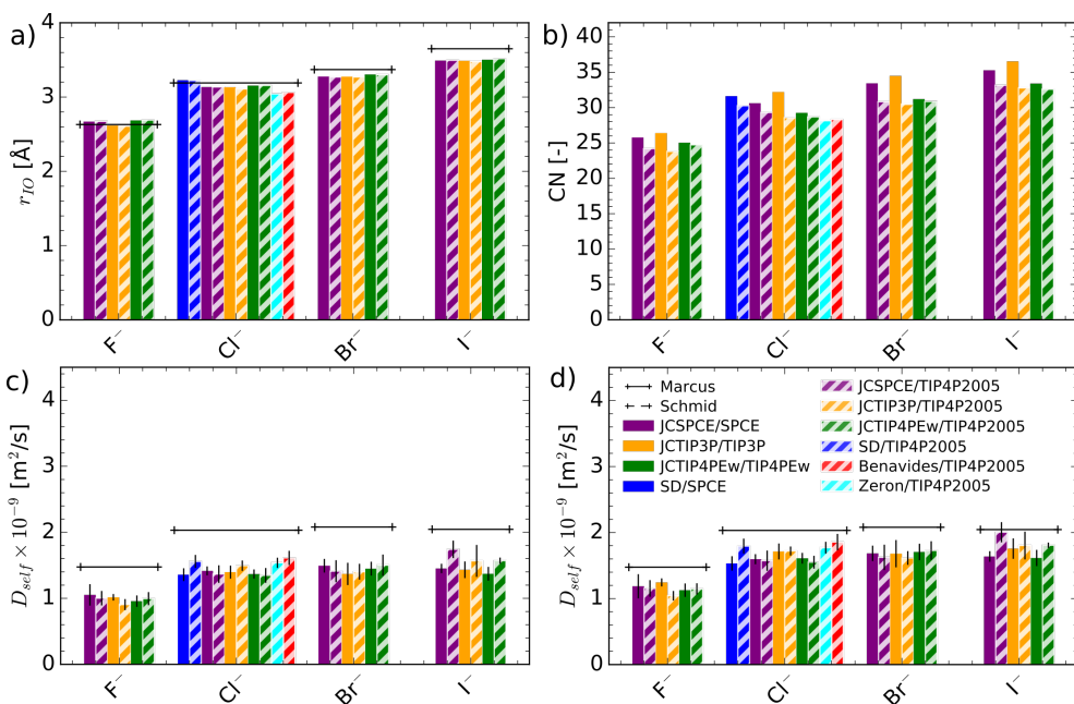
Figure 2.10: Radius (a) and coordination number (b). Scaled diffusion coefficients by \eta_{model}/\eta_{exp} (c) and by D_{i,exp}/D_{i,model} (d) for monovalent anions.
