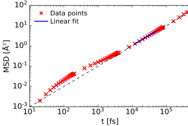
Figure 2.2: MSD obtained for a single SD Na + ion in TIP4P/2005 water. Ballistic regime is found at t < 10 , and linear regime at t > 10 ps. Linear regression was done from 10 to 50 ps obtaining the slope. Coefficients of determination for the regression were above 0.999 for all simulations.
