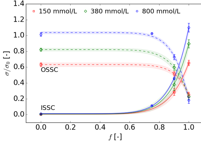
Figure 4.6: Relative charge contribution of ions ( \text{Ca}^{2+} and \text{Cl}^- ) forming ISSC ( \sigma_{\text{ISSC}}/\sigma_0 and \sigma_{\text{OSSC}}/\sigma_0 ) as a function of the scaling parameter f for bulk \text{CaCl}_2 concentrations of 150, 380 and 800 mmol/L. The confidence intervals are 68 %.
