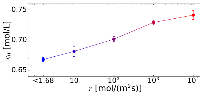
Figure 5.1: Ion concentration c_0 in the center of the channel as a function of the protolysis reaction rate r .
