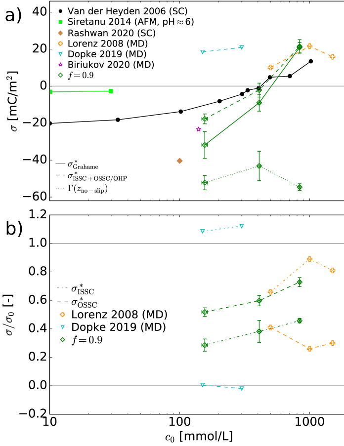
Figure 4.11: (a) Differing definitions of the effective surface charge density \sigma_{\text{Grahame}}^* , \Gamma(z_{\text{no-slip}}) and \sigma_{\text{ISSC}+\text{OSSC}}^* \approx \sigma_{\text{OHP}}^* from experiments and MD simulations at varying concentrations. (b) The relative charge contributions of \sigma_{\text{ISSC}}^* and \sigma_{\text{OSSC}}^* for various MD studies. The confidence intervals are 68 %.
