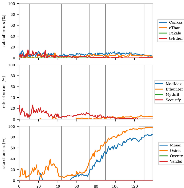
Fig. 6 Tool errors over time. Each data point shows the percentage of errors reported by the tools, in bins of 100k blocks. Mythril, Oyente and Vandal had no errors
