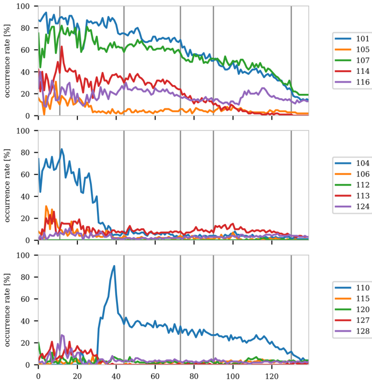
Fig. 4 SWC classes over time. Each data point shows the percentage of bytecodes flagged with a specific weakness, in bins of 100k blocks
