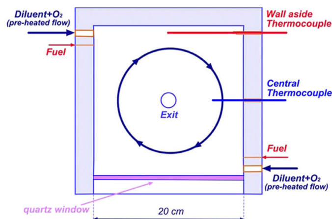
Fig. 15. Scheme of the prismatic combustion chamber designed by Sorrentino et al. [90].
