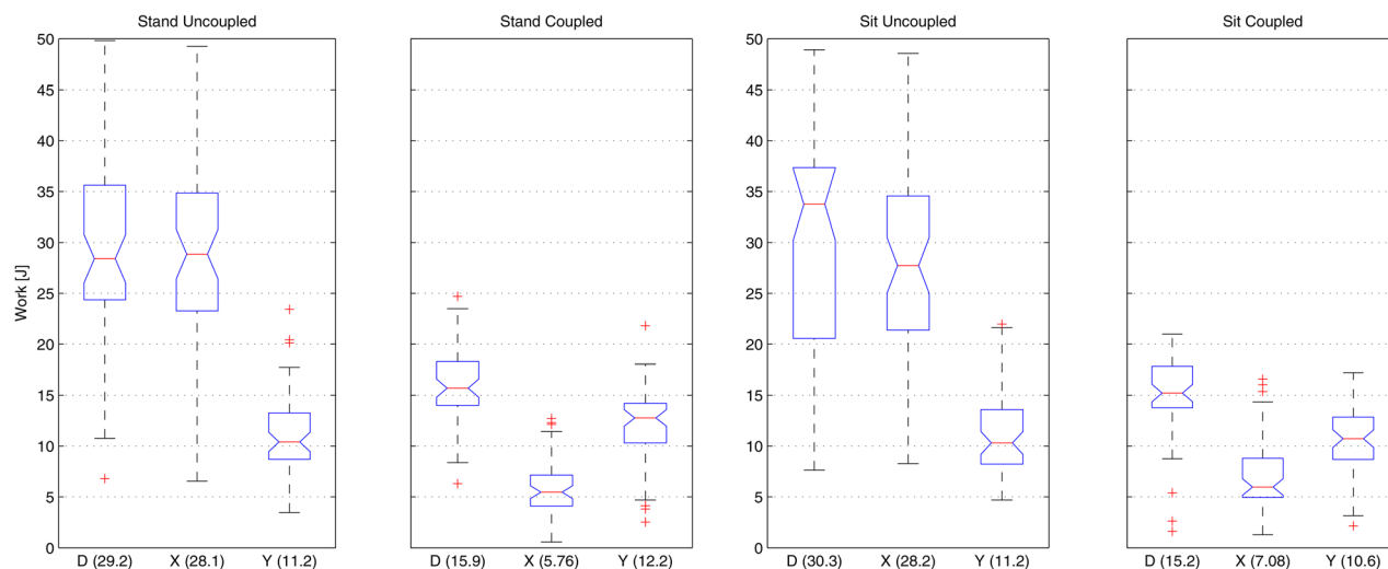
Fig. 6 The average work values in Joule for all participants, grouped by posture, state, and movement type; diagonal ( D ), X and Y . Nonoverlapping notches show that medians differ at a 5% significance level. Thus, it can be observed that there is no difference between postures and that there is difference between system states except for the y -movements. As a reference, the work value of 25 J is approximately equivalent to lifting 2.5 kg to a height of 1 m.
