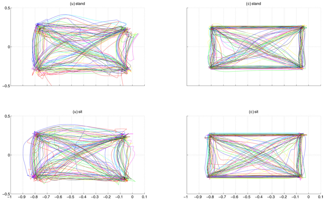
Fig. 4 The movement paths of the end-effector of all participants, plotted on the movement-board. The movements with the conventional uncoupled mechanism are plotted at the left and with the conceptual coupled mechanism at the right. The upper figures are of the movements performed in a standing posture and the lower figures of the performance in a sitting posture. It can be observed that the perpendicular translations in the coupled mechanism create straight movement paths, whereas the uncoupled mechanism is moved along curved paths.
