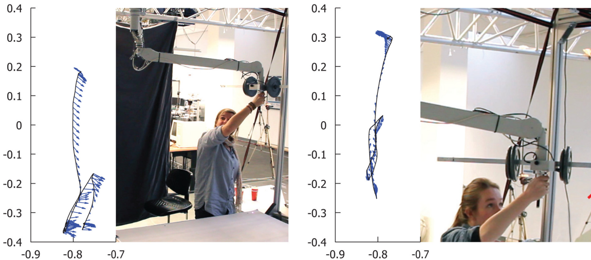
Fig. 8 The traveled path is depicted to the left of a video still of two occurring problems; (left) relative high friction in the suspension causes the participant to repeatedly overshoot the target caused by the build-up of force to overcome friction in precise movements. (Right) Rotations of the end-effector causes collisions or entanglement of the cross beam with the setup frame. The depicted case is the most severe, in which the suspension is completely retracted before the movement can be completed.
