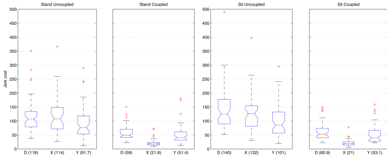
Fig. 10 Jerk cost of for various scenarios depicted as boxplots
