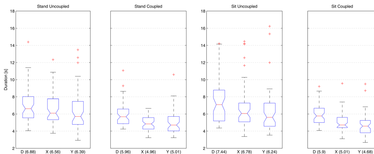
Fig. 7 The duration of each movement for all participants, grouped by posture, system state, and movement type; diagonal ( D ), X , and Y . It can be observed that the duration of movements made with the coupled mechanism is shorter on average. However, the notches denote the 5% significance, which shows that the duration difference is insignificant for y -movements.
