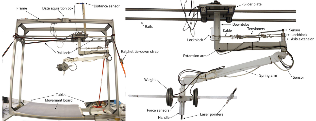
Fig. 1 The experimental setup on the left and a close-up of the prototype on the right. The experimental setup is photographed in the conventional uncoupled state. The close-up is of the coupled state.
