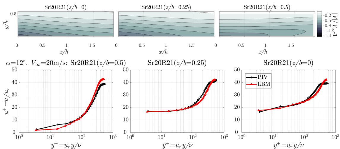
Fig. 17 Contours of velocity variation along the three spanwise locations of Fig. 2 in the top row; bottom: experimental boundary-layer profiles of u^+ as from experimental and numerical data. Boundary-layer fit with k=0.40 , B=5 , u_\tau=0.50 m/s (White 2006)
