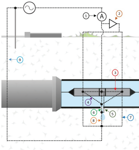
Figure 2. The model; an electrical circuit of the geo-electrical measurement system. The left side shows the nodes and their mutual connections, the right side shows how the admittances are related in a typical field application. The corresponding colours and numbers indicate the links between the components on both sides of the figure.
