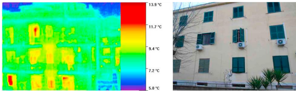
Fig. 5. Infrared and normal picture of South Elevation.
