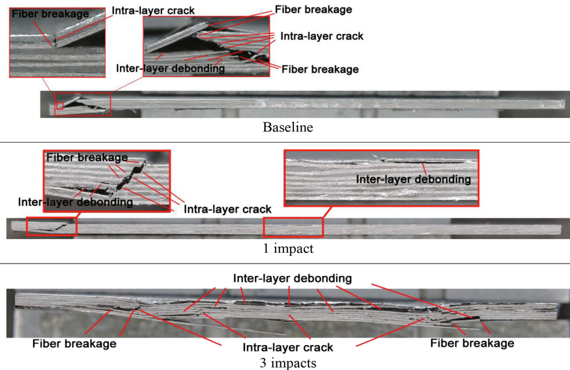
Fig. 10. Microscopy images of the cross section of NCF specimen after CAI test.
