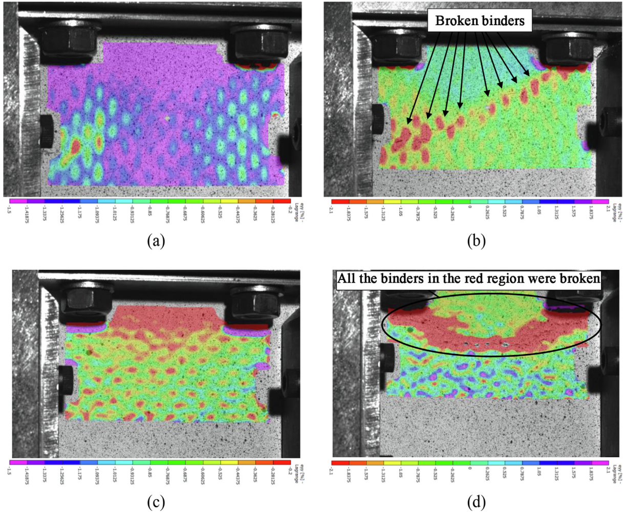
Fig. 17. The eyy strain (in the loading direction) distribution in ORT-PW architecture for a) the linear elastic segment of the load–displacement curve where no damage exists (z-binding yarns are visible), b) the final failure of baseline specimen, c) the linear elastic segment of the load–displacement curve where no damage exists (z-binding yarns are visible) and d) the final failure of single-impact specimen.
