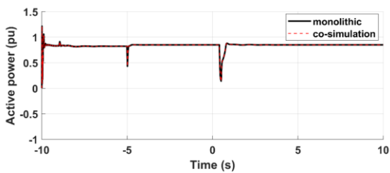
Fig. 5.b: The active power output of the WT
