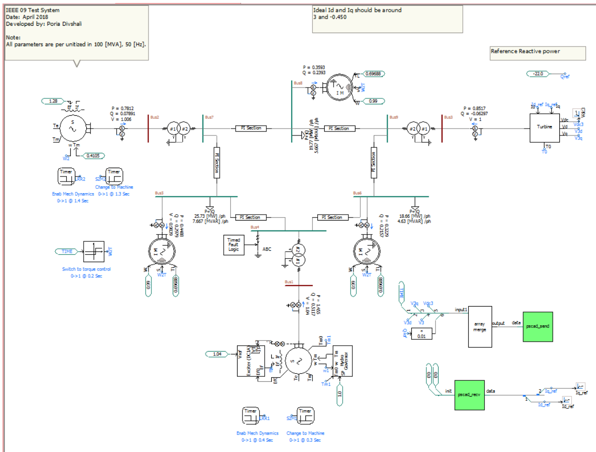
Fig. 4: The dynamic model of IEEE 9 bus system, implemented in PSCAD
