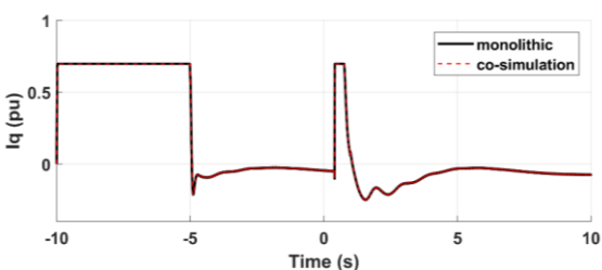
Fig. 5.e: The reference current ( I_q ) of the WT
