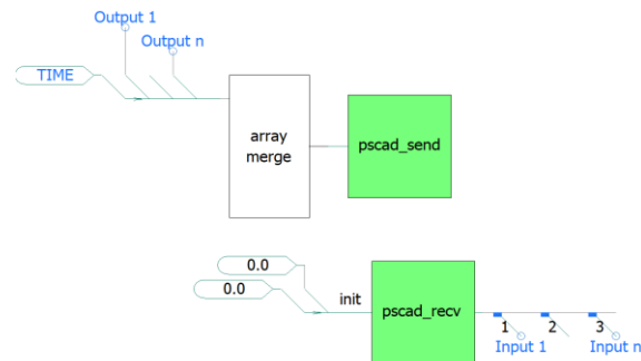
Fig. 3: the PSCAD co-simulation interface
