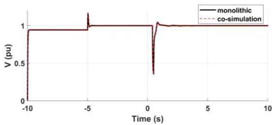
Fig. 5.a: The output voltage of the WT
