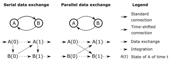
Fig. 2: Data exchange schemes possible in mosaik.
