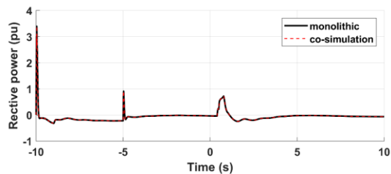
Fig. 5.c: The reactive power output of the WT
