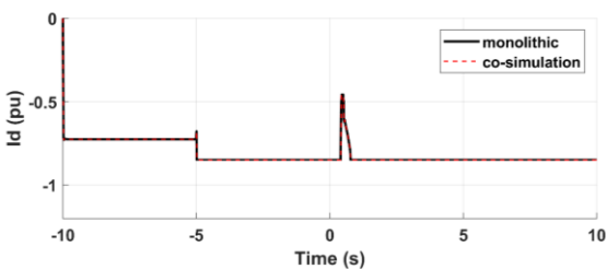
Fig. 5.d: The reference current ( I_d ) of the WT
