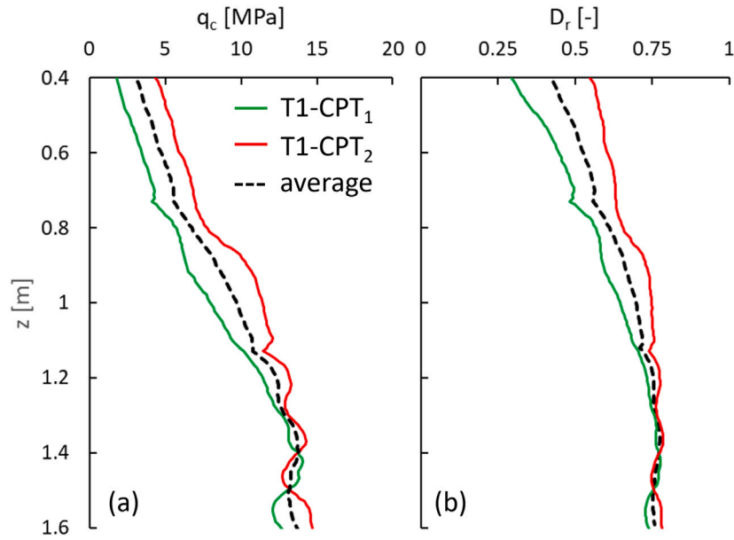
Fig. 3. Test 1: (a) cone resistance as a function of depth and (b) the corresponding relative density.
