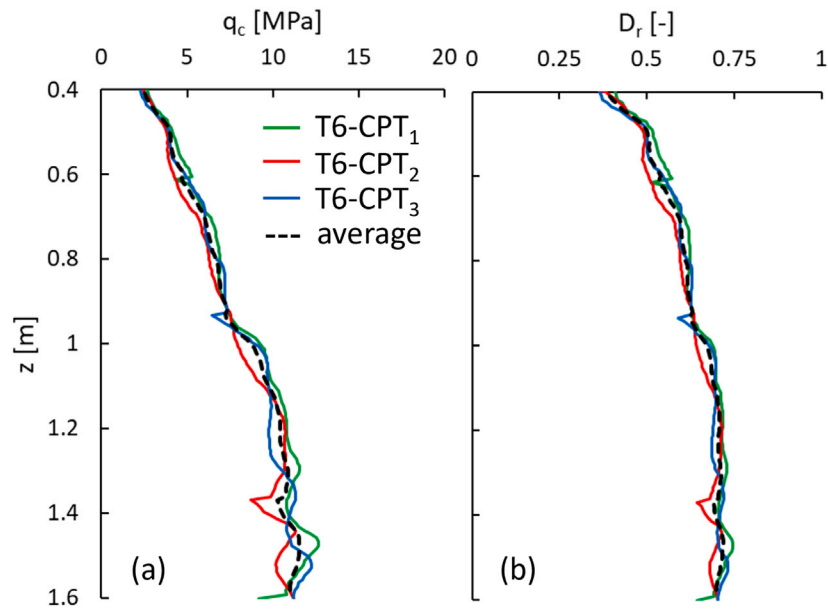
Fig. 4. Test 6: (a) cone resistance as a function of depth and (b) the corresponding relative density.
