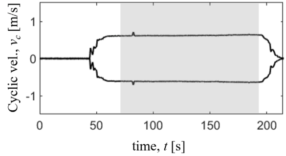
Fig. 9. Time-history response of pile T1: Envelope of maximum and minimum cyclic velocities. The gray background highlights the interval in which driving is ongoing.
