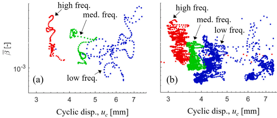
Fig. 19. Evolution of \bar{\beta} with cyclic displacement ( u_c ). (a) “fast” installation and (b) “slow” installation. High frequency ( f > 30 Hz), low frequency ( f < 20 Hz), and medium frequency for values in between. Note that the vertical axis is presented on a logarithmic scale to emphasize variation across orders of magnitude. .
