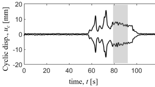
Fig. 12. Time-history response of pile T6: Envelope of maximum and minimum cyclic displacements. The gray background highlights the interval in which driving is ongoing.
