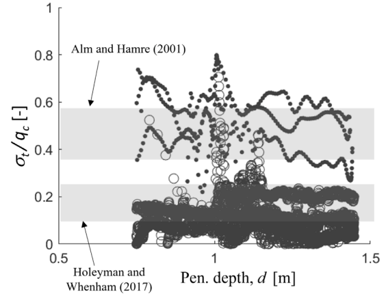
Fig. 17. Evolution of the ratio \sigma_t/q_c with penetration depth. Filled markers for fast installation and unfilled for slow installation .
