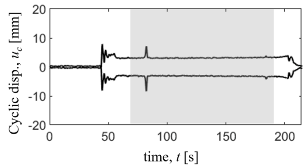
Fig. 10. Time-history response of pile T1: Envelope of maximum and minimum cyclic displacements. The gray background highlights the interval in which driving is ongoing.
