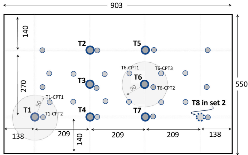
Fig. 2. The location of CPTs and piles (T1–T7) for set #1, and pile T8 for set #2.
