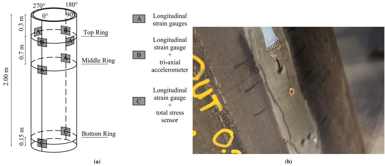
Fig. 5. (a) Schematic representation of the pile instrumentation. (b) A close-up photograph of the total pressure sensor installed at the bottom ring of the pile.
