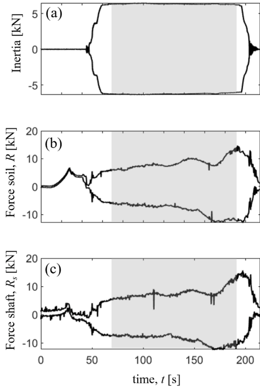
Fig. 13. Time-history response of pile T1. Envelope of maximum and minimum forces: (a) inertia forces, (b) soil reaction forces, and (c) shaft reaction forces. The gray background highlights the interval in which driving is ongoing.
