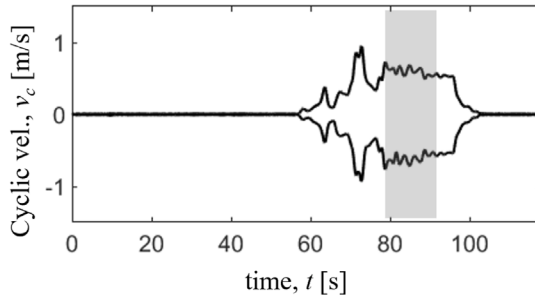
Fig. 11. Time-history response of pile T6: Envelope of maximum and minimum cyclic velocities. The gray background highlights the interval in which driving is ongoing.
