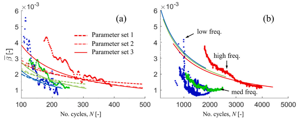
Fig. 22. Evolution of \bar{\beta} number of cycles ( N ). (a) “fast” installation and (b) “slow” installation. The comparison includes experimental data and back-calculated analytical models: Eq. (18) for “fast” installation and Eq. (20) for “slow” installation. Different colors represent different frequency ranges, from low to high.
