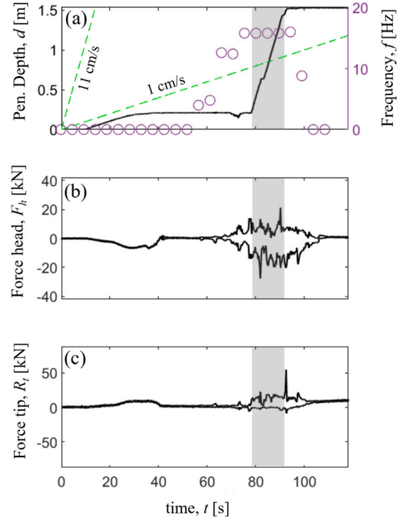
Fig. 8. Time-history response of pile T6: (a) Penetration, (b) envelope of maximum and minimum forces at the pile head, and (c) envelope of maximum and minimum forces at the pile tip. The gray background highlights the interval in which driving is ongoing.
