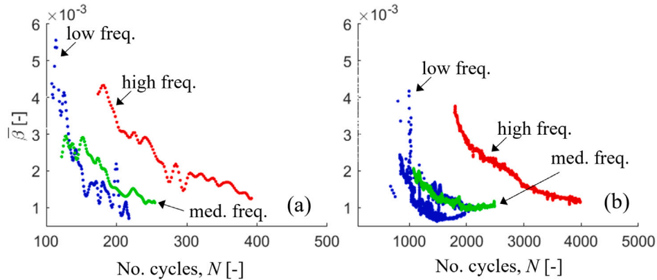
Fig. 20. Evolution of \bar{\beta} with number of cycles ( N ). (a) “fast” installation and (b) “slow” installation. High frequency ( f > 30 Hz), low frequency ( f < 20 Hz), and medium frequency for values in between.
