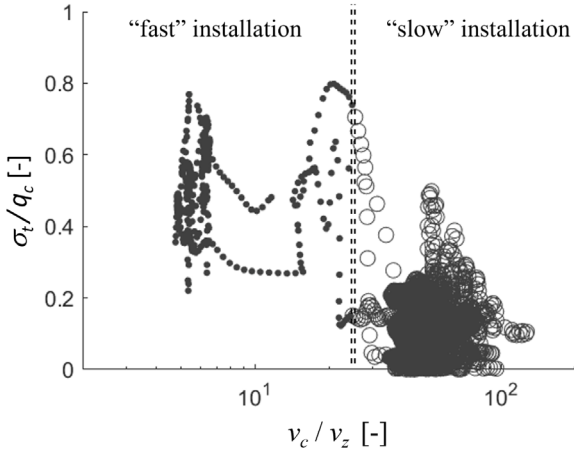
Fig. 16. The ratio \sigma_t/q_c as function of v_c/v_z . Filled markers for fast installation and unfilled for slow installation .
