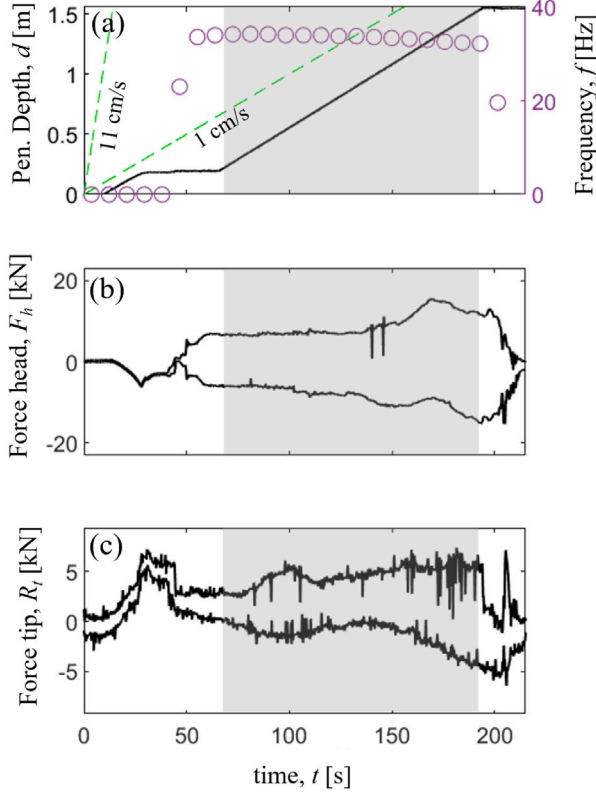
Fig. 7. Time-history response of pile T1: (a) Penetration, (b) envelope of maximum and minimum forces at the pile head, and (c) envelope of maximum and minimum forces at the pile tip. The gray background highlights the interval in which driving is ongoing.
