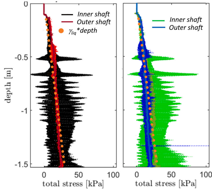
Fig. 15. Results of the total stress installed on pile T8, on the inner and outer shaft as function of the sensor depth.
