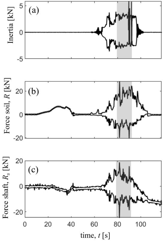
Fig. 14. Time-history response of pile T6. Envelope of maximum and minimum forces: (a) inertia forces, (b) soil reaction forces, and (c) shaft reaction forces. The gray background highlights the interval in which driving is ongoing.
