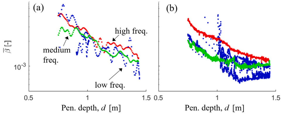
Fig. 18. Evolution of \bar{\beta} with penetration depth ( d ). (a) “fast” installation and (b) “slow” installation. High frequency ( f > 30 Hz), low frequency ( f < 20 Hz), and medium frequency for values in between. Note that the vertical axis is presented on a logarithmic scale to emphasize variation across orders of magnitude. .
