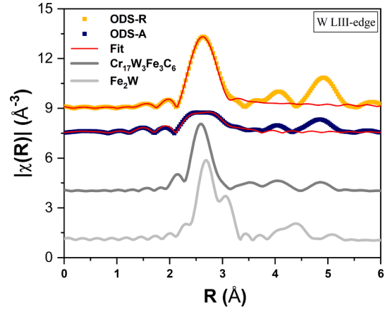
Fig. 15. Fourier transform magnitude of k^2 -weighted EXAFS oscillations on the W LIII-edge for ODS-R, ODS-A, their respective fits, and the simulated WFe_2 and Cr_{17}W_3Fe_3C_6 . First W-Fe scattering path from Fe_2W has been used for phase correction. Experimental data were fitted in the R range between 2.1 and 3.4 Å.
