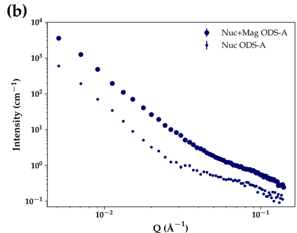
Fig. 4. (a) A 2D SANS scattering pattern contour plot with the magnetic field perpendicular to the incident beam on ODS-A. (b) Nuclear plus magnetic and nuclear components for ODS-A obtained from (a).
