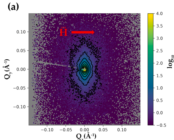
Fig. 4. (a) A 2D SANS scattering pattern contour plot with the magnetic field perpendicular to the incident beam on ODS-A. (b) Nuclear plus magnetic and nuclear components for ODS-A obtained from (a).
