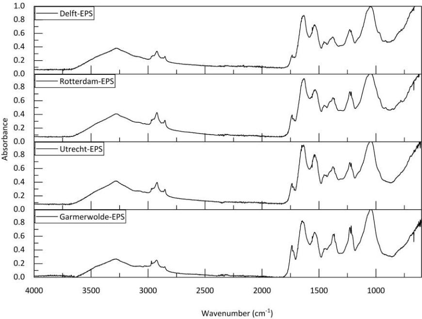
Figure S2 FTIR spectra of EPS samples from different sludge.
