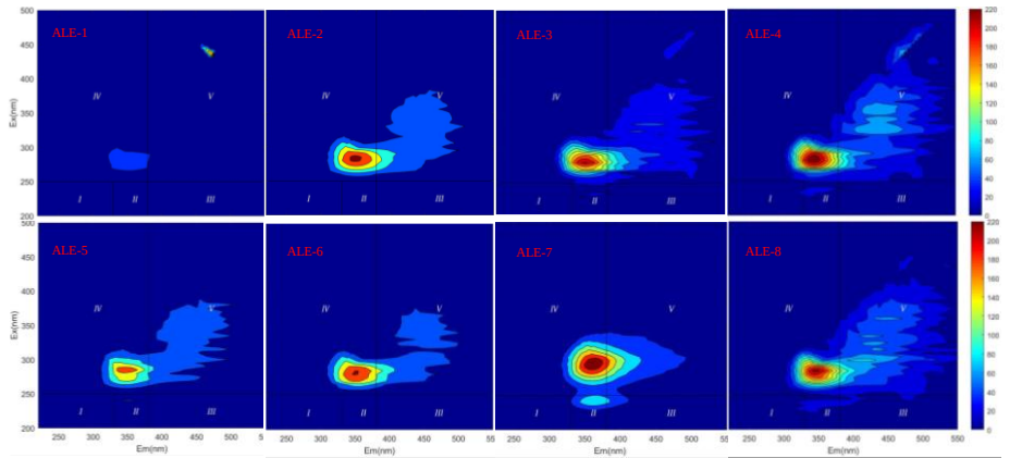
Figure S4 Three-dimensional excitation-emission matrix (3D-EEM) of extracellular biopolymers. (EEM spectra were collected with subsequent emission (Em) spectra from 220 to 550 nm at 1 nm increment by varying the excitation (Ex) wavelength from 200 to 500 nm at 5 nm increments. Ex and Em slits were maintained at 5 nm and the scanning speed was set at 1,200 nm/min for all the measurements.)
