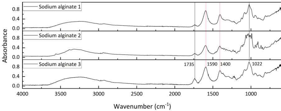
Figure S5 FTIR spectrum of three commercial sodium alginates.
