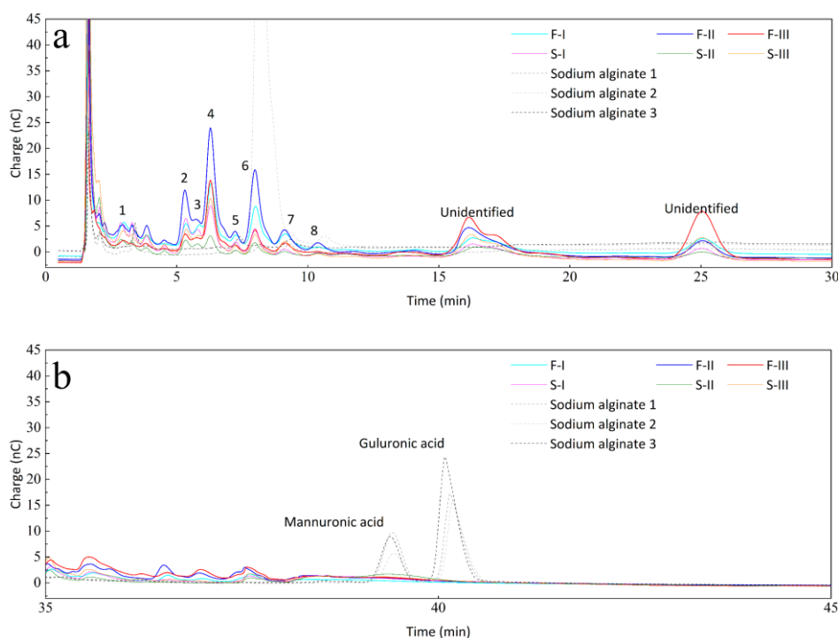
Figure 1 HPAEC-PAD chromatograms of standards, different EPS fractions and three commercial alginates after complete acid hydrolysis. Sugar monomer speaks: 1-fucose, 2-galactosamine, 3-rhamnose, 4-glucosamine, 5-galactose, 6-glucose, 7-xylose and 8-mannose. Sodium alginates concentration was at 50 mg/L. (a) retention time at 0-30 min with the eluent of 2 mM sodium hydroxide, (b) retention time at 35-45 min with the eluent of 50 mM sodium acetate plus 200 mM sodium hydroxide. The baseline drifted at 30-35 min periods as the eluent was changed. F I-III and S I-III represent Fractions I~III and Ethanol supernatants I~III, respectively.
