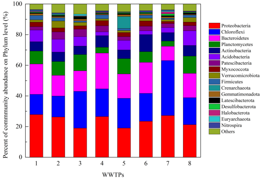
Figure 2 Abundance of microorganisms at the phylum levels from the different wastewater treatment plants (WWTPs).
