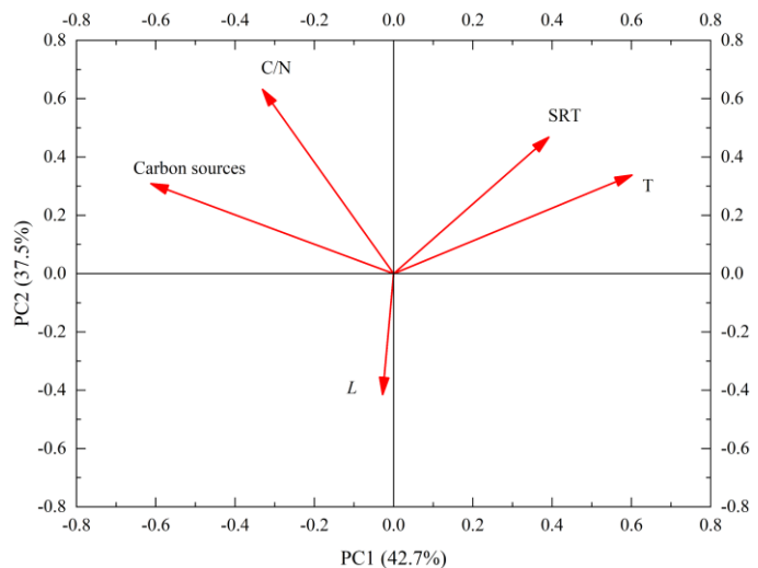
Figure S5 Loading biplot for principal component analysis (PCA) for the correlations of operational parameters with the alginate like extracellular polymers (ALE) formation.
