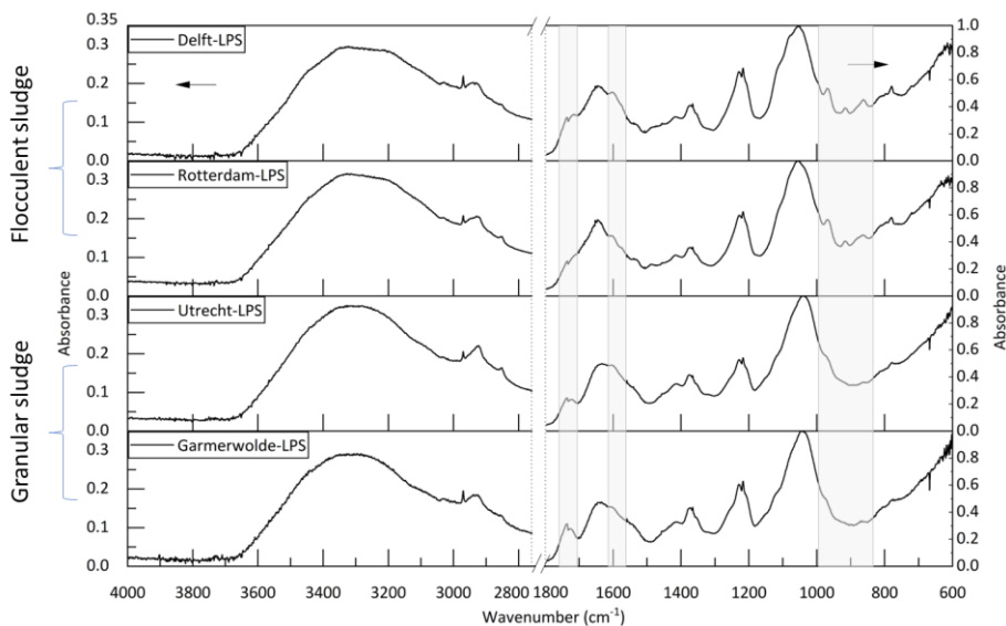
Figure 3 FT-IR spectra of lipopolysaccharides (LPS) isolated from flocculent sludge (Delft and Rotterdam) and granular sludges (Utrecht and Garmerwolde) (wavenumber from 4000\text{--}2800 and 1800\text{--}600\text{ cm}^{-1} ).
