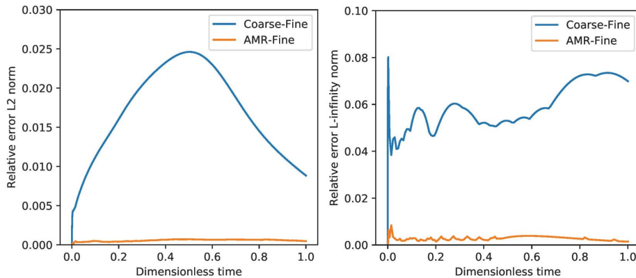
Figure 9 L2 norm (left) and L-infinity norm (right) of the difference between the coarse model and the fine model, and between the AMR model and the fine model, both relative to the fine-scale solution, for the homogeneous model with unstructured gridding from figures 7 to 8.
