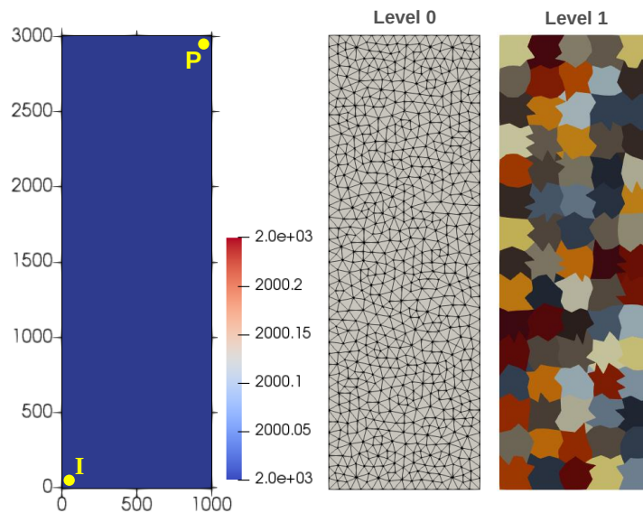
Figure 7 Hierarchical grid of the unstructured homogeneous model. Left figure: permeability field with reservoir dimensions and well locations; middle figure: level 0, the finest level of refinement, with unstructured gridding; right figure: coarser level, level 1 where each color represents a coarse cell.
