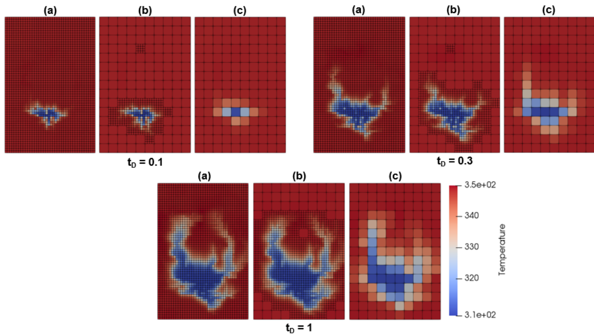
Figure 12 Temperature solution of the heterogeneous model with low net-to-gross ratio at three different times: at t_D = 0.1 , 0.3 and 1 . (a) is the fine-scale solution (level 0); (b) is the AMR solution; (c) is the coarse-scale solution (level 1).
