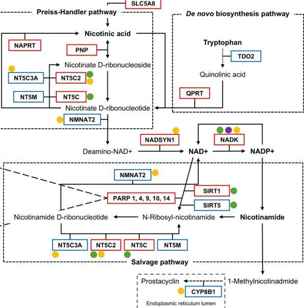
Fig. 3 Overview of the differentially expressed genes and DNA (hydroxy)methylation levels within the TRP metabolic pathway and NAD pathway. Within the TRP metabolic pathway, a total of 12 genes exhibited significant differential gene expression, while 20 genes were differentially expressed within the NAD pathway. Genes exhibiting up-regulation in expression are highlighted with red box, whereas those with down-regulation are indicated by blue box. Genes with altered DNA (hydroxy)methylation levels are denoted by circular markers, with distinct colors representing specific modifications: 5mC (green), 5hmC (purple), and 5uC (orange)
