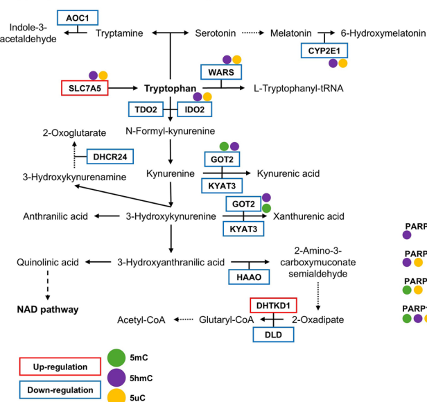
Fig. 3 Overview of the differentially expressed genes and DNA (hydroxy)methylation levels within the TRP metabolic pathway and NAD pathway. Within the TRP metabolic pathway, a total of 12 genes exhibited significant differential gene expression, while 20 genes were differentially expressed within the NAD pathway. Genes exhibiting up-regulation in expression are highlighted with red box, whereas those with down-regulation are indicated by blue box. Genes with altered DNA (hydroxy)methylation levels are denoted by circular markers, with distinct colors representing specific modifications: 5mC (green), 5hmC (purple), and 5uC (orange)
