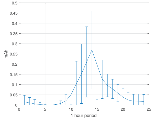
Figure 3: Window Sill - Averaged energy reading over 378 days for each 1 hour period in a day
