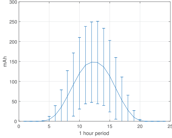
Figure 5: Outdoors - Averaged energy reading over 365 days for each 1 hour period in a day
