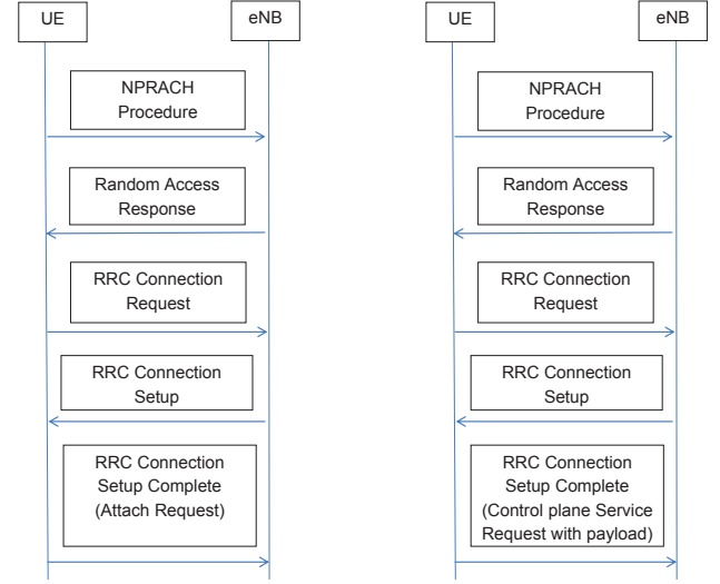
Figure 1: Attach Request and Payload exchange procedures
