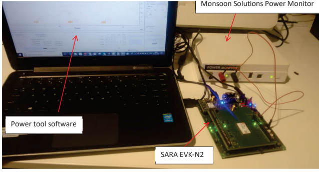
Figure 2: Current measurement using Monsoon Solutions power monitor tool
