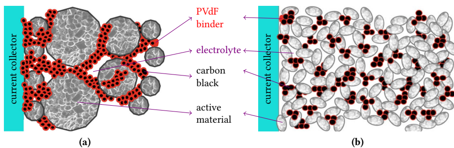
Fig. 1.2. Schematic of the composition of two popular commercial Li-ion battery cathodes: (a) an NMC cathode and (b) an LFP cathode [1]. The porous cathode consists of active materials, conductive carbon black, and PVdF polymer binder. The two types of cathodes differ in the choice of active materials: NMC electrodes use Lithium Nickel Manganese Cobalt oxide ( LiNiMnCoO_2 ) while LFP takes Lithium Iron Phosphate ( LiFePO_4 ). The electrolyte fills in the pores.
