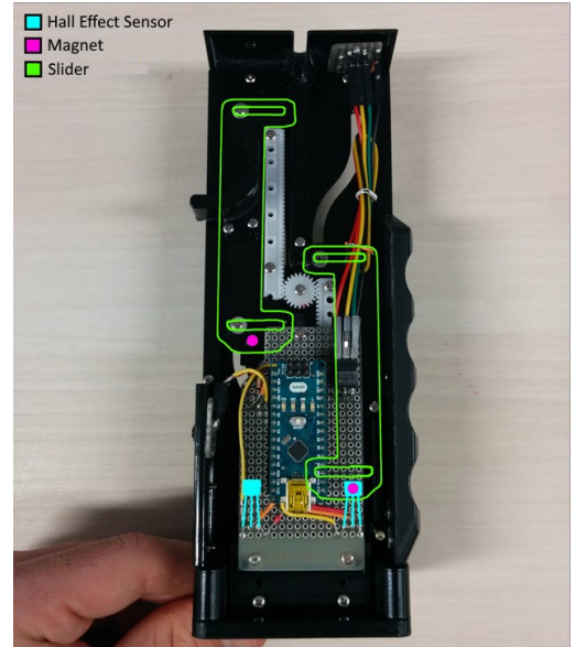
Fig. 5. Trigger mechanism for image capture. Hall effect sensors (cyan) detect the presence of magnets (magenta) attached to the pen- or microscope-slider (green). For example, if the pen reaches the bottom, i.e. if dotting occurs, the sensor sends a signal to the CPU to indicate a dotting action.
