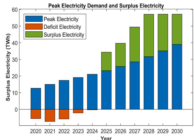
Fig. 6. Calculated SE with year.
