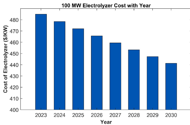
Fig. 5. Cost of 100 MW Electrolyzer with year.
