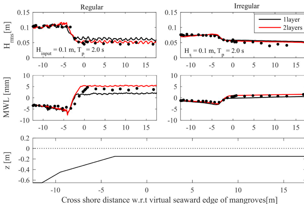
Fig. 7. Comparisons between numerical model with 1 vertical layer (black line) and numerical model with 2 vertical layers (red line) and physical model (markers) for both regular (left hand side) and irregular wave (right hand side). (For interpretation of the references to colour in this figure legend, the reader is referred to the Web version of this article.)
