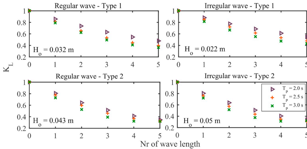
Fig. 4. Effective wave transmission K_L in cases of sparse mangroves, different wave periods: T_p = 2 s (black triangles), T_p = 2.5 s (red pluses) and T_p = 3 s (green crosses). (For interpretation of the references to colour in this figure legend, the reader is referred to the Web version of this article.)
