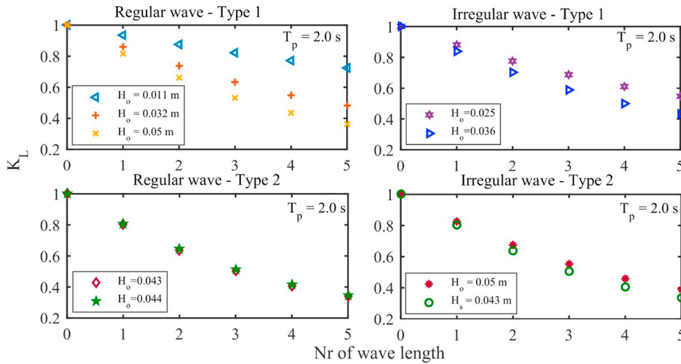
Fig. 5. Effective wave transmission K_L in cases of sparse vegetation, wave period of 2s, different wave height.
