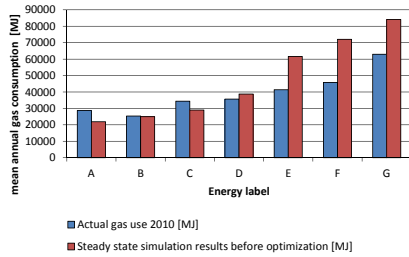
FIG. 6.10 comparison actual versus simulated gas consumption before optimisation (calculated with steady state simulation method), based on data from WoON energiemodule 2012
