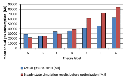
FIG. 6.7 comparison actual versus simulated gas consumption (calculated with steady state method), based on data from WoON energiemodule 2012)
