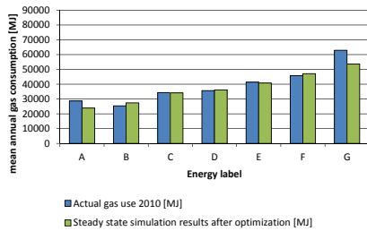
FIG. 6.12 comparison actual versus simulated gas consumption after optimisation (calculated with steady state simulation method), based on data from WoON energiemodule 2012
