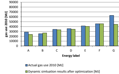
FIG. 5.16 Actual versus theoretical gas consumption calculated with dynamic simulation method after optimisation - sample
