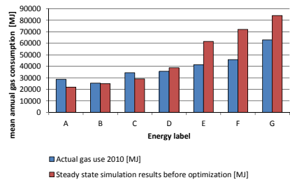
FIG. 5.13 Actual versus theoretical gas consumption calculated with steady state simulation method before optimisation - sample
