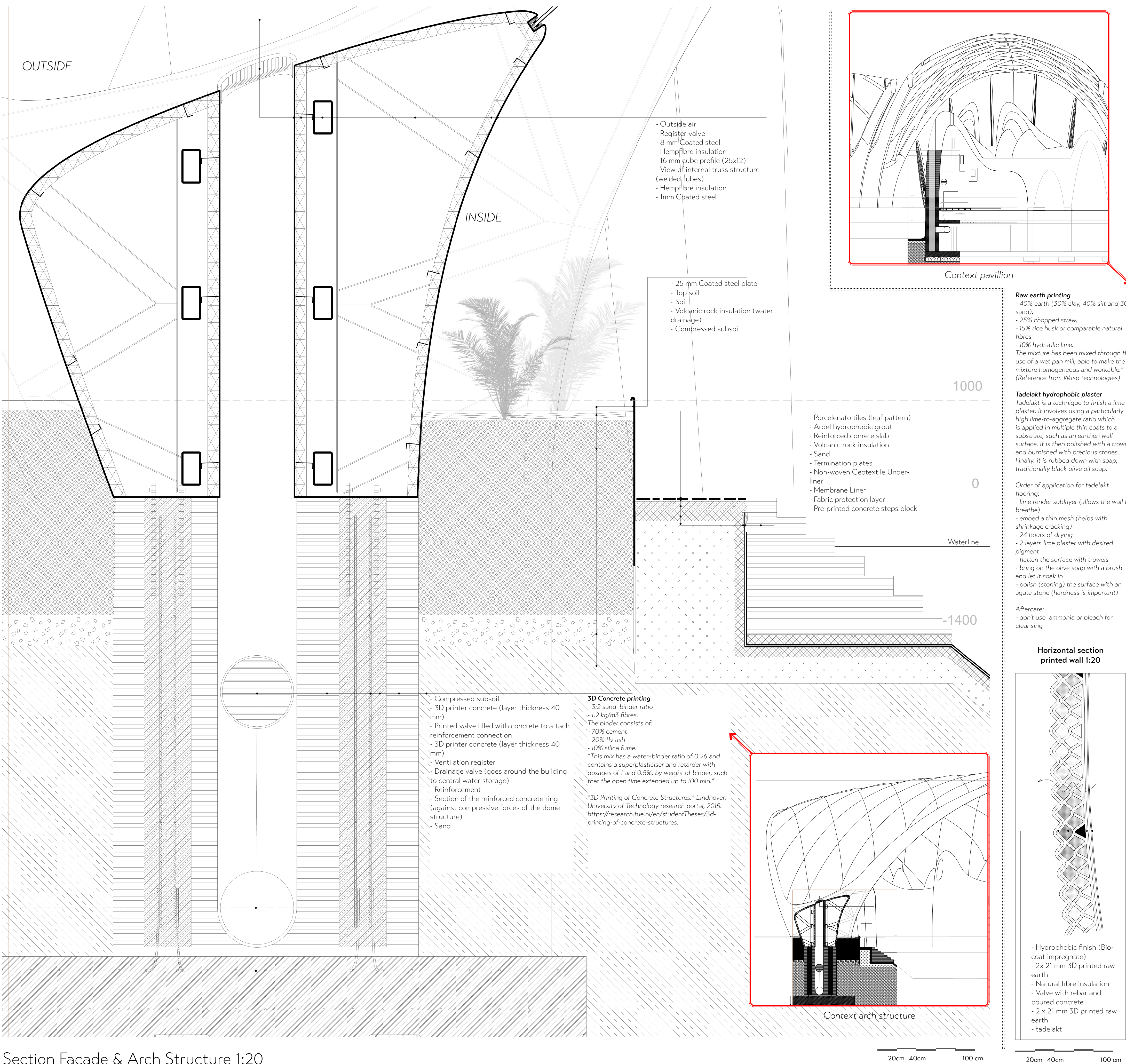
Section Facade & Arch Structure 1:20
