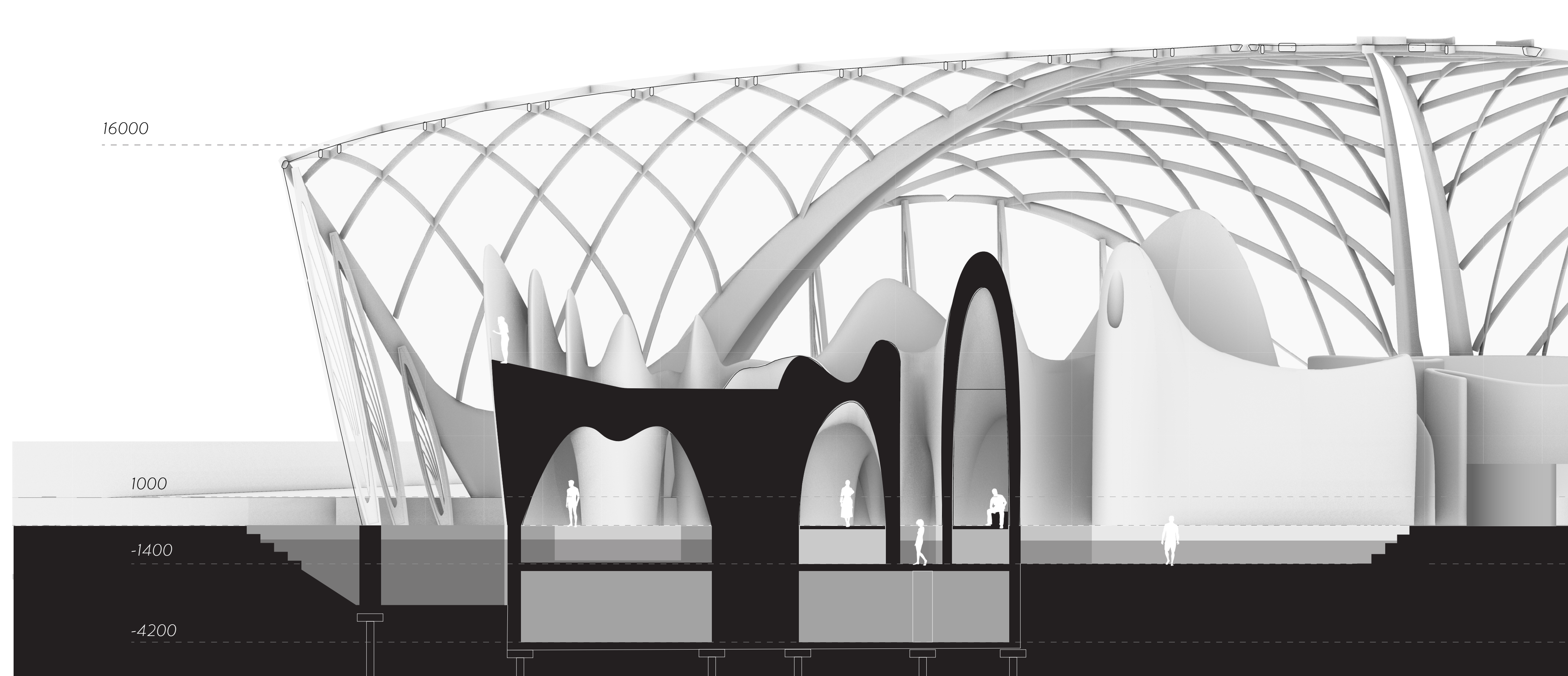
Section H 1:100
