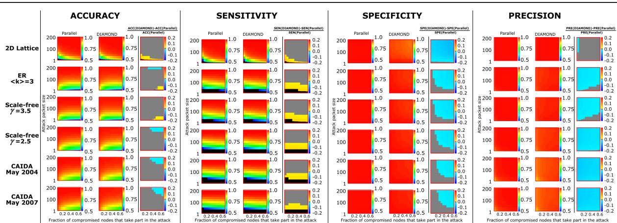
Fig. 6 Values of accuracy, sensitivity, specificity, and precision for uniformly distributed traffic. For the parallel algorithm, we use the upper threshold, s_{10}
