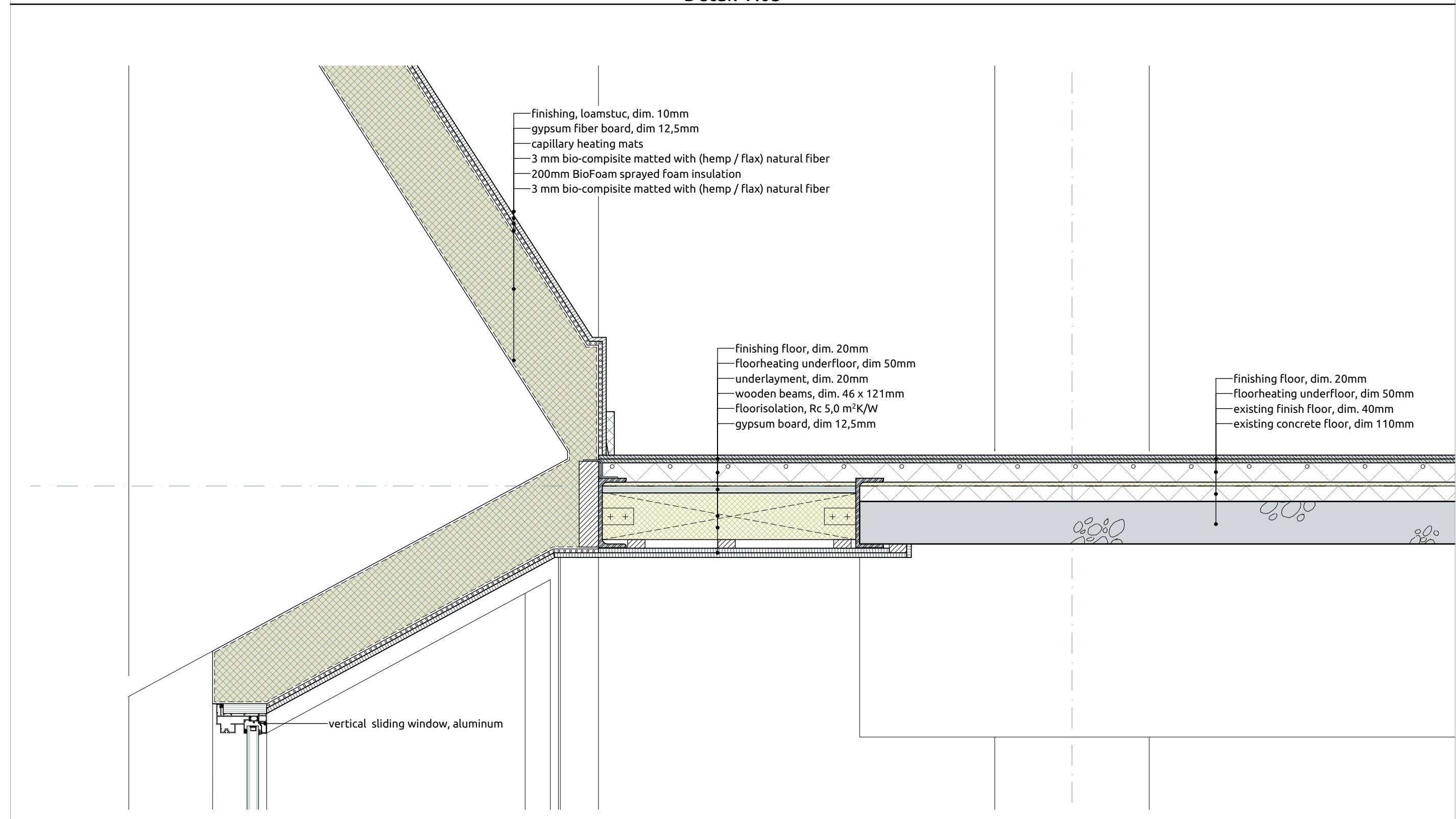
Detail V.02
