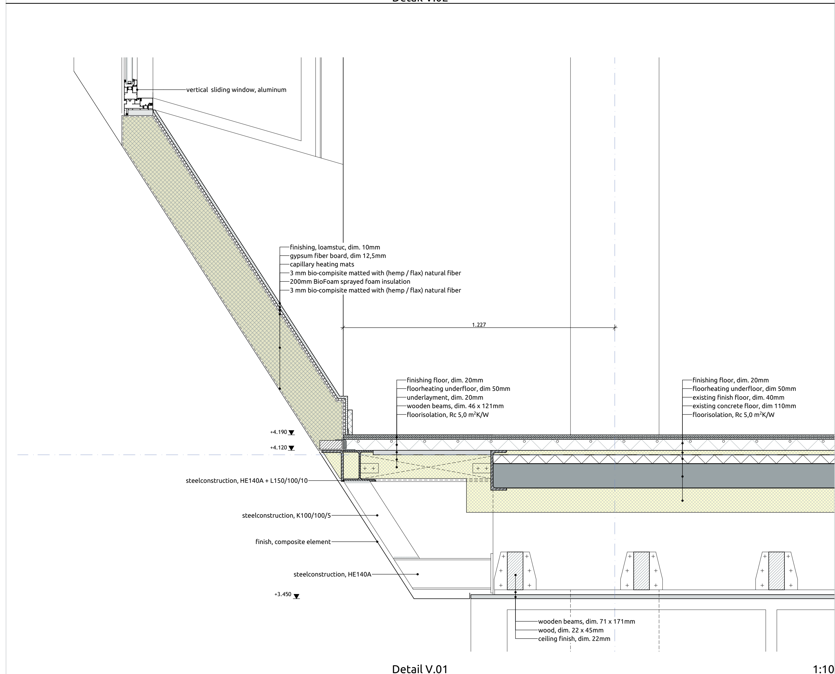
Detail V.01
