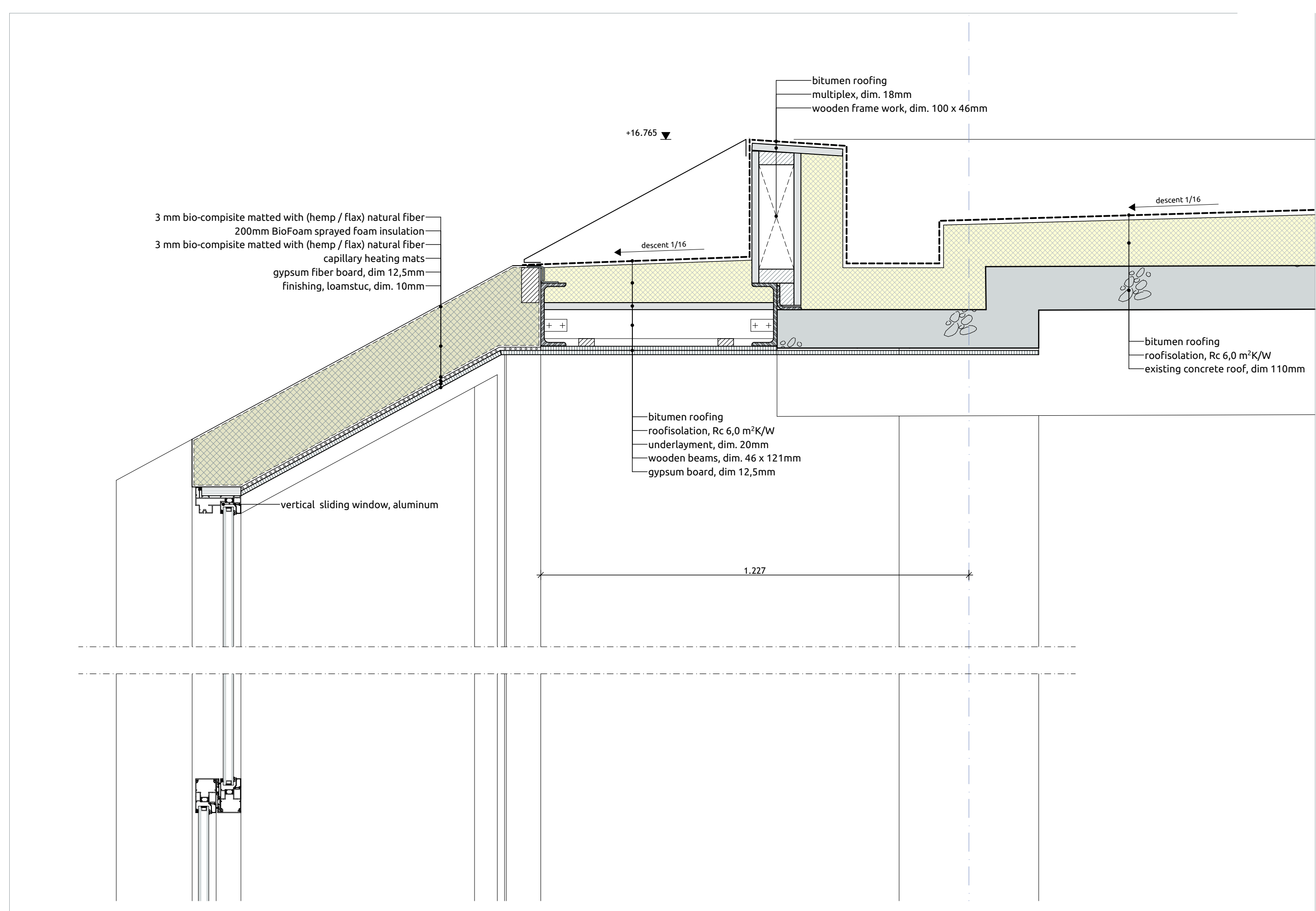
Detail V.03
