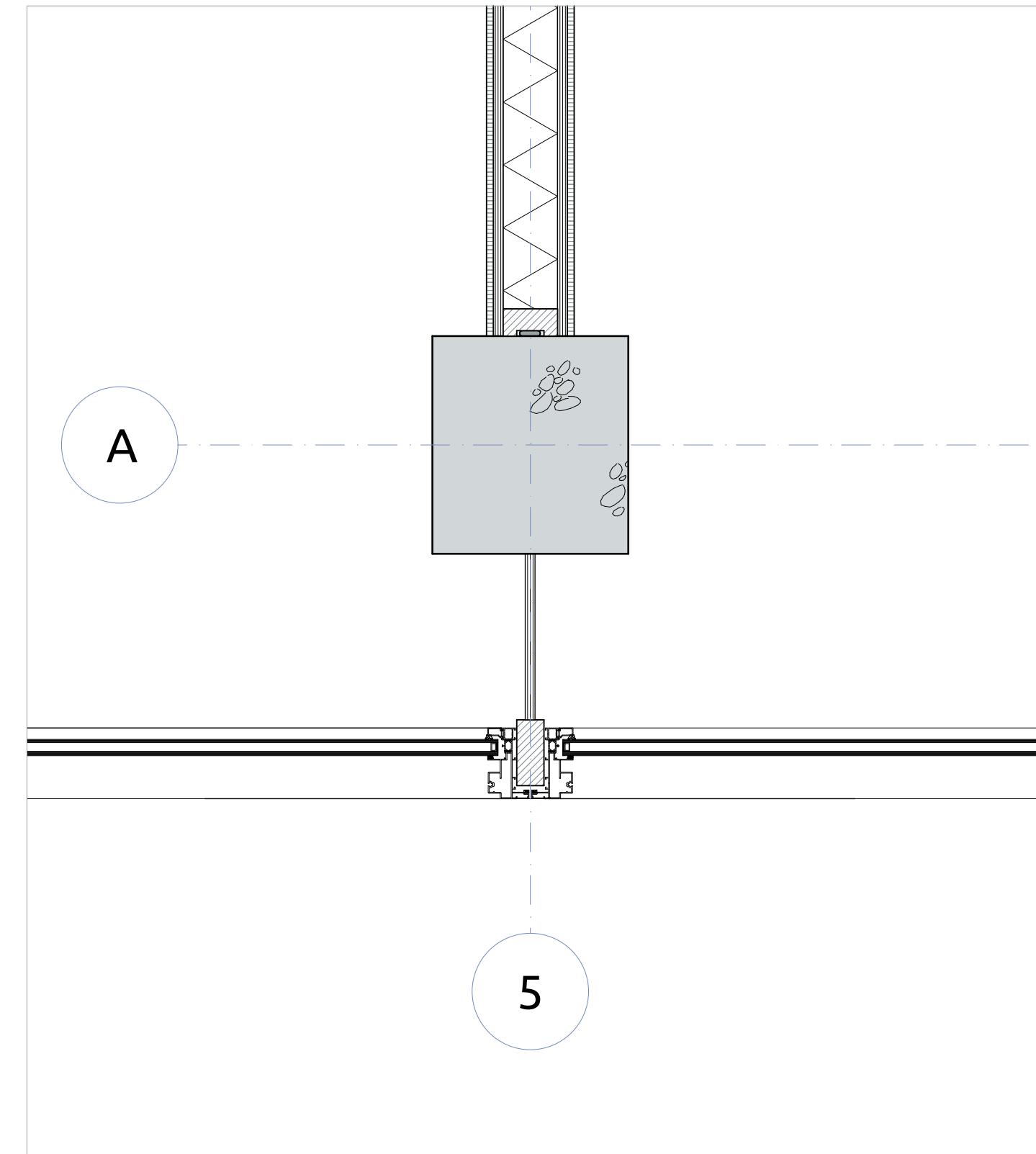
Detail H.01
