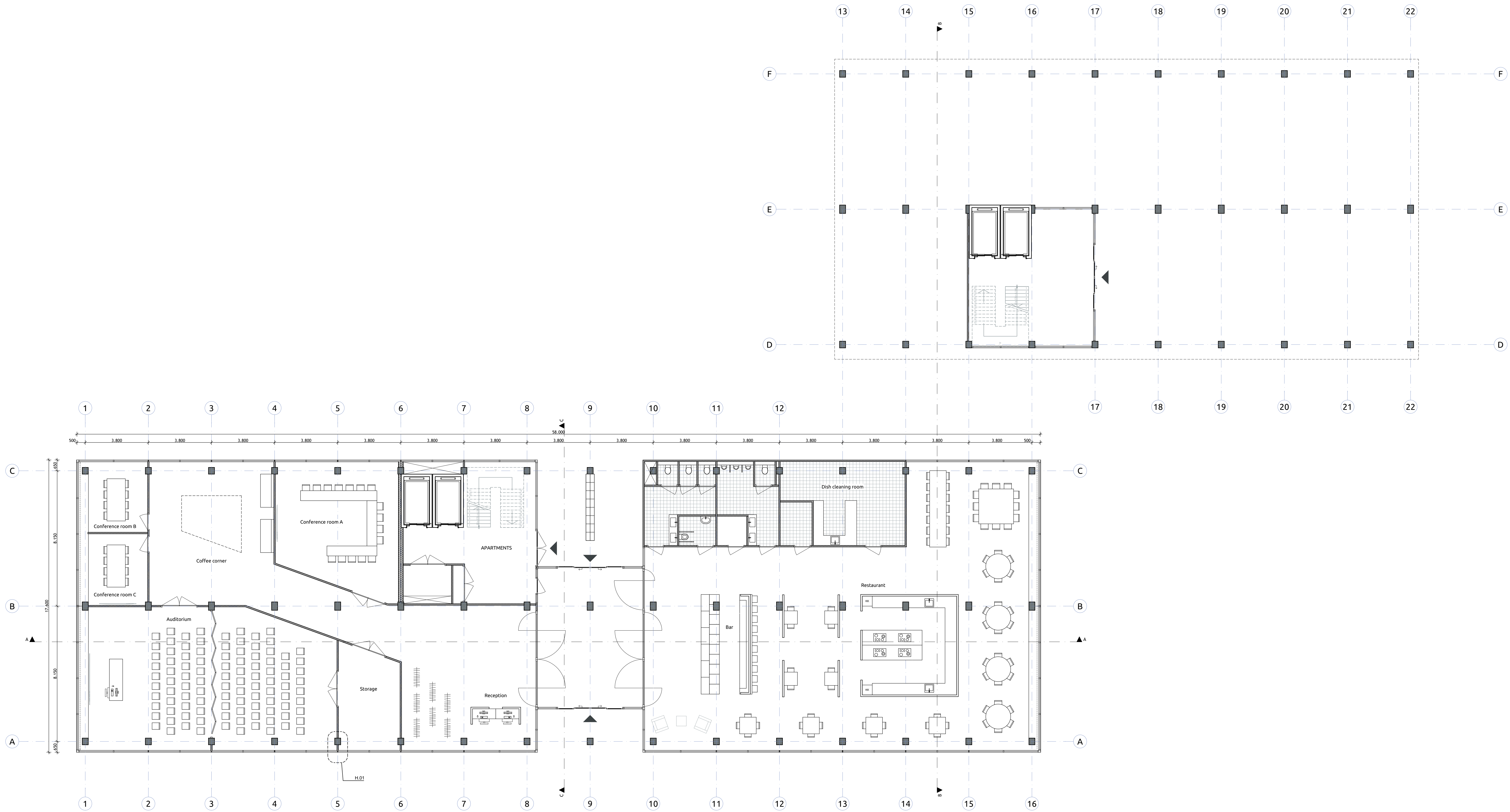
Ground floor
