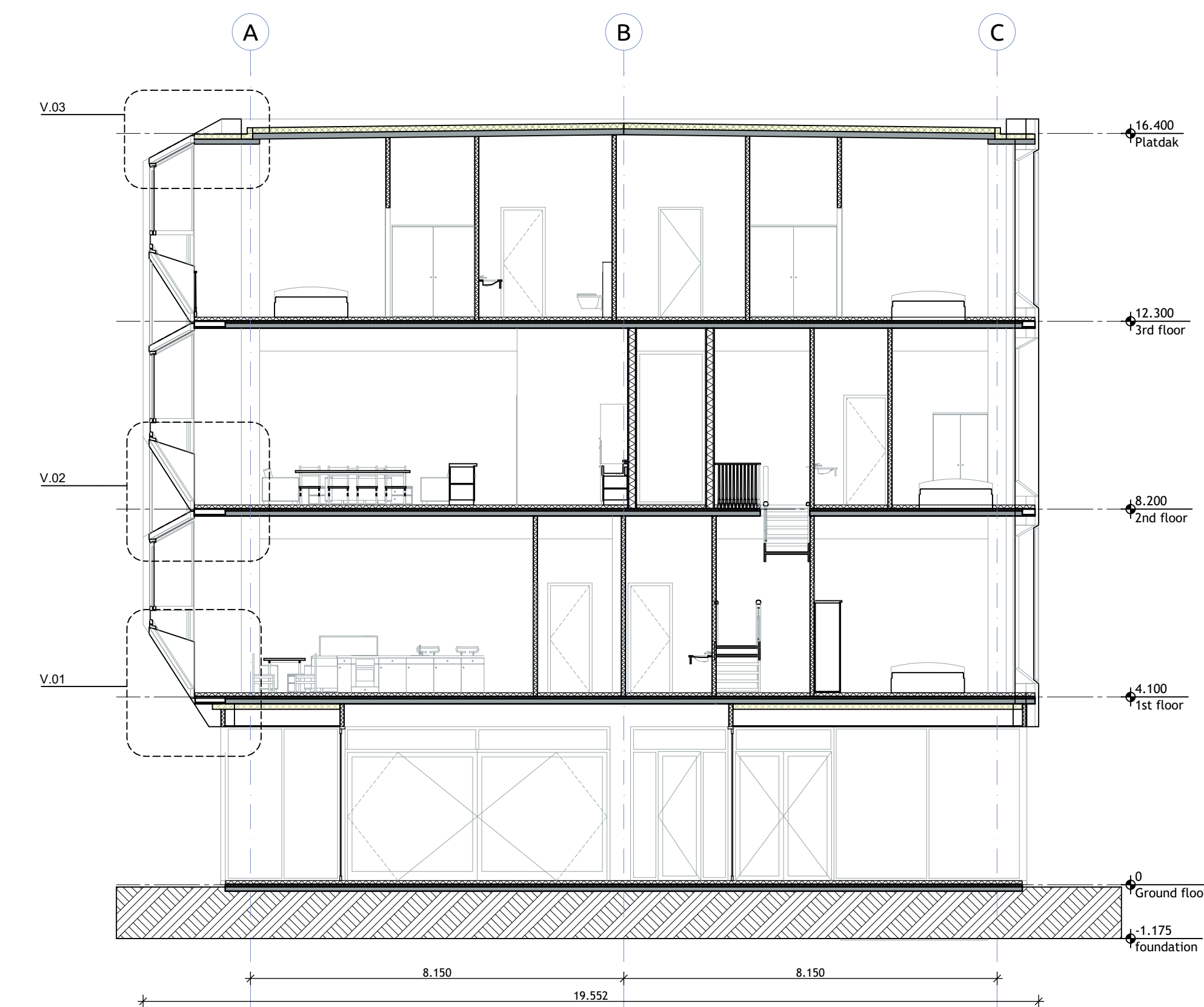
Cross section C - C
