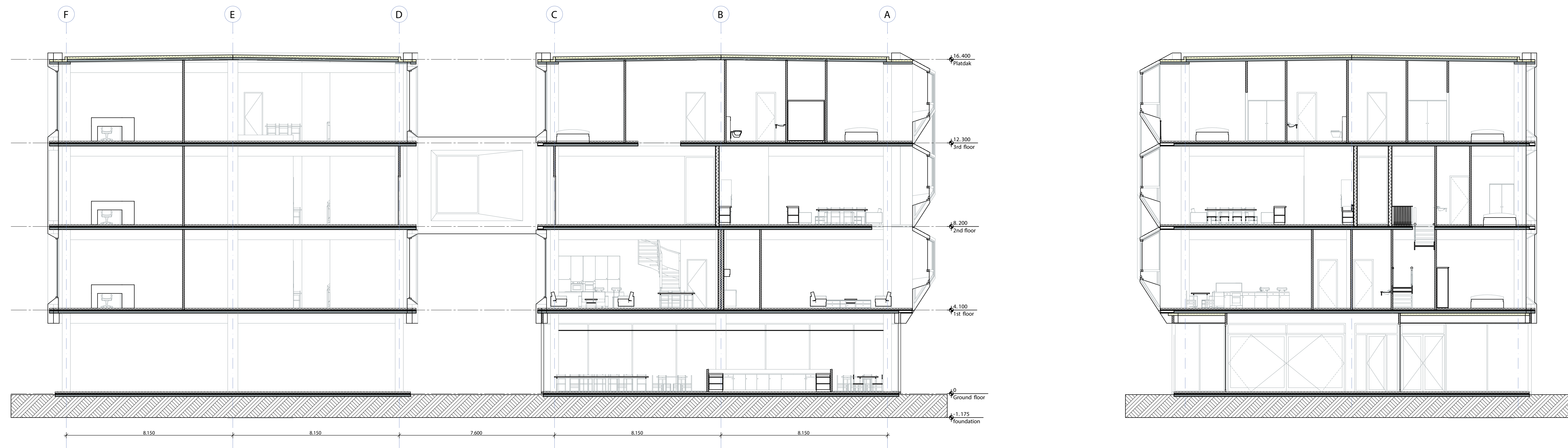
Cross section B - B
