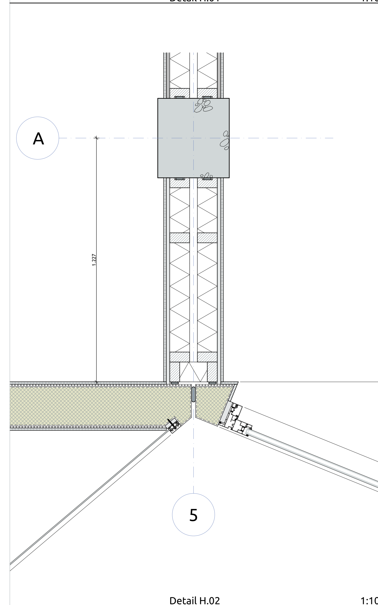
Detail H.02
