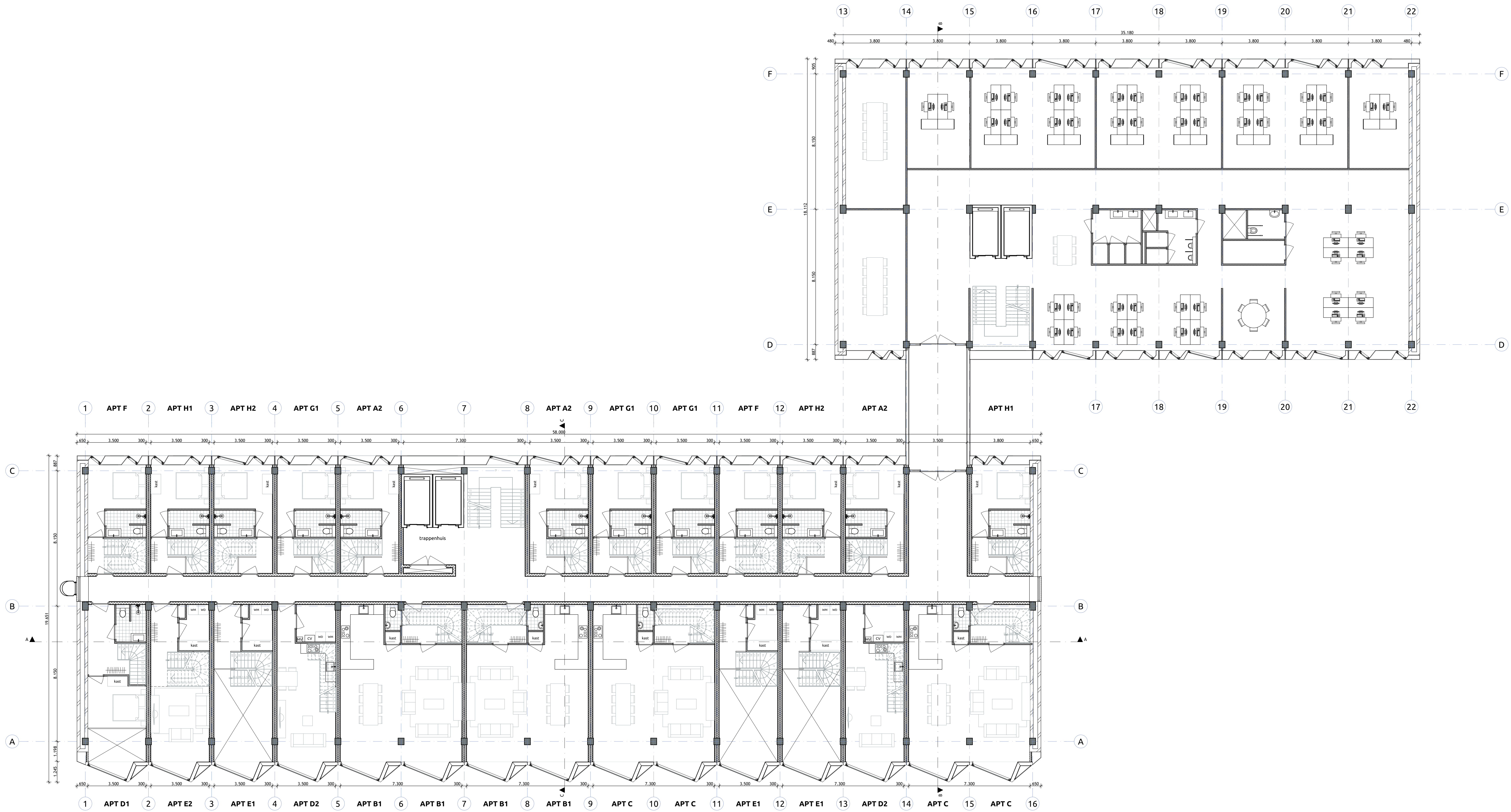
2nd floor
