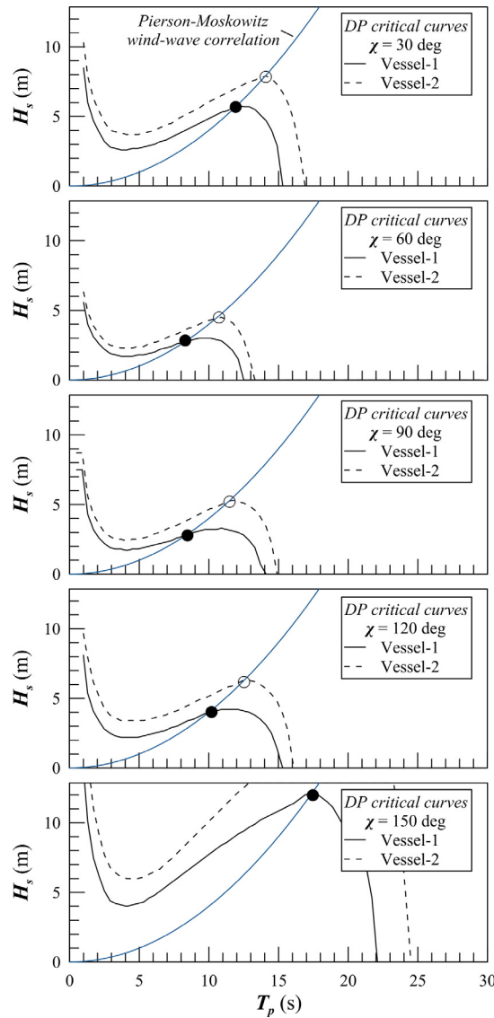
Fig. 5. Correspondence between site-specific DP critical curves and deterministic DP capability plots using the Pierson-Moskowitz wind-wave correlation for Vessel-1 and Vessel-2.
