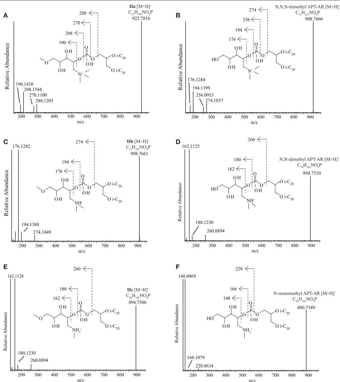
FIGURE 5 | UHPLC-HRMS MS 2 spectra with structures and fragmentations indicated for (A) N,N,N -trimethyl aminomethoxypentane (trimethyl APT-Me, IIa ), (B) N,N,N -trimethyl aminopentane (trimethyl APT), (C) N,N -dimethyl aminomethoxypentane (dimethyl APT-Me, IIb ), (D) N,N -dimethyl aminopentane (dimethyl APT), (E) N -monomethyl aminomethoxypentane (monomethyl APT-Me, IIc ), (F) N -monomethyl aminopentane (monomethyl APT). i-C 20 , C 20 isoprenoid chain.
