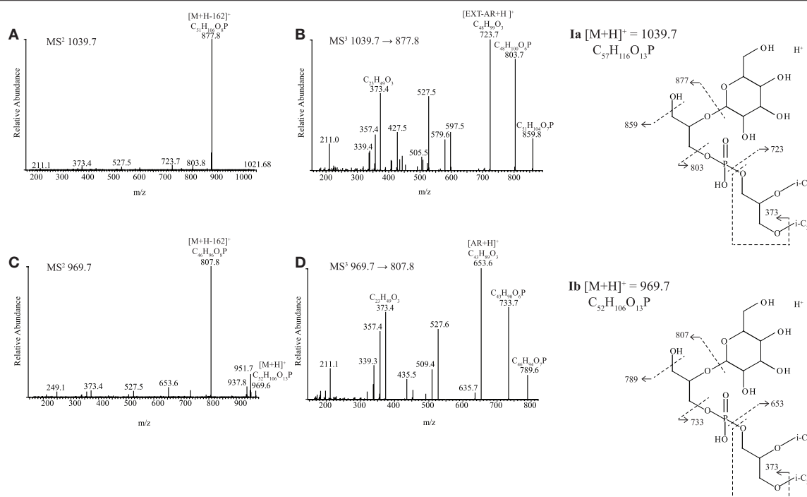
FIGURE 4 | HPLC-ITMS 2 and MS 3 spectra with inserts of structure with fragmentations indicated for (A,B) Ia PG-Gly-EXT-AR and (C,D) Ib PG-Gly-AR. i-C 20 , C 20 isoprenoid chain; i-C 25 , C 25 isoprenoid chain.
