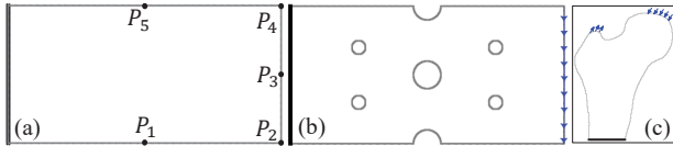
Figure 7: The 2D solid objects used in our experiments. Blue arrows indicate the load conditions. (a) Cantilever with fixed left edge, discretized into 250 \times 500 finite elements. Points P_1, \dots, P_5 indicate the positions where different loads are applied. (b) Perforated plate, adapted from the cantilever. (c) Slice through a 3D CT-scan of a femur, fixed at the bottom and discretized into 182 \times 140 finite elements.
