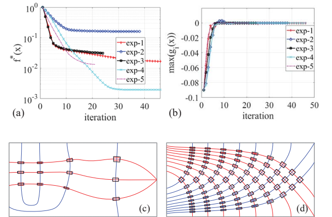
Figure 12: Top: Convergence analysis for all 2D experiments. (a) Normalized objective function. (b) Constraint function. Bottom: Comparisons of seed elements before and after optimization, for the 2nd (c) and 3rd (d) test case. Elements with colored edges depict the initial seed elements, black edges indicate optimized elements.
