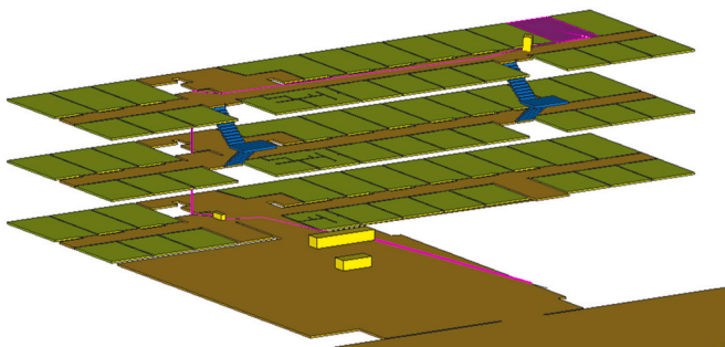
Fig. 12. An obstacle-avoiding path.
