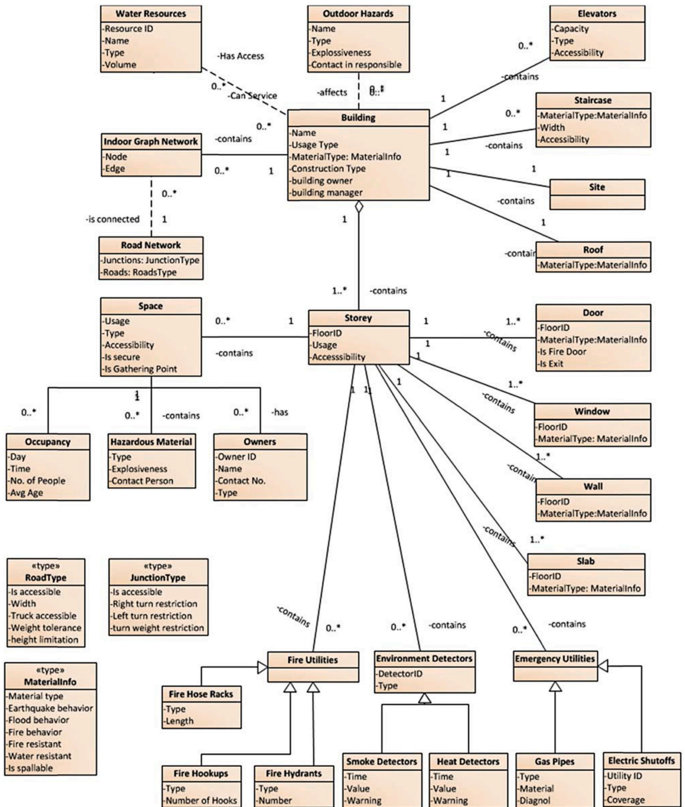
Fig. 15. The data model of IESM ([76]).
