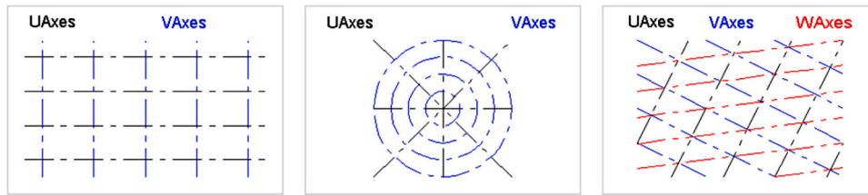
(b) Three types of IfcGrid
