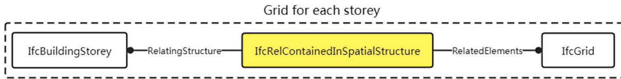
(a) The relationship between IfcStorey and IfcGrid
