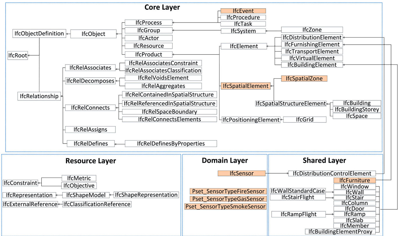
Fig. 2. The main IFC classes supporting indoor navigation. The highlighted classes are newly added in IFC4.
