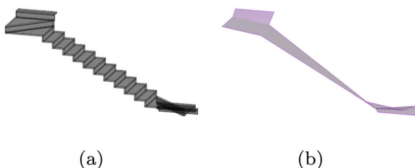
Fig. 20. Boundary creation from an IfcStair instance. (a) A stair as a composite solid; and (b) the stair as a 3D polygon.
