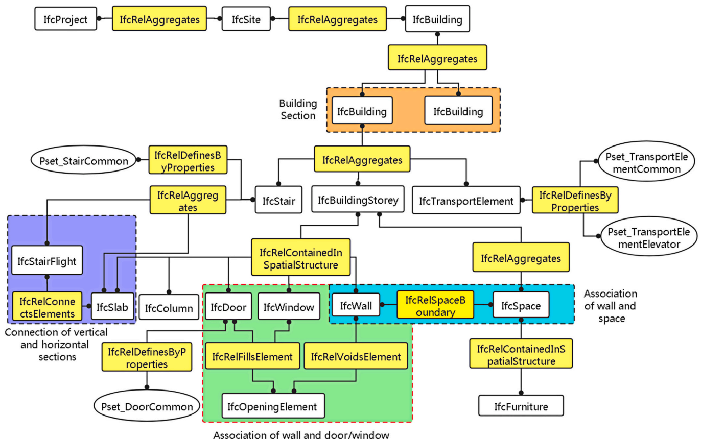
Fig. 19. The suggested minimum set of IFC classes to derive indoor navigation models.
