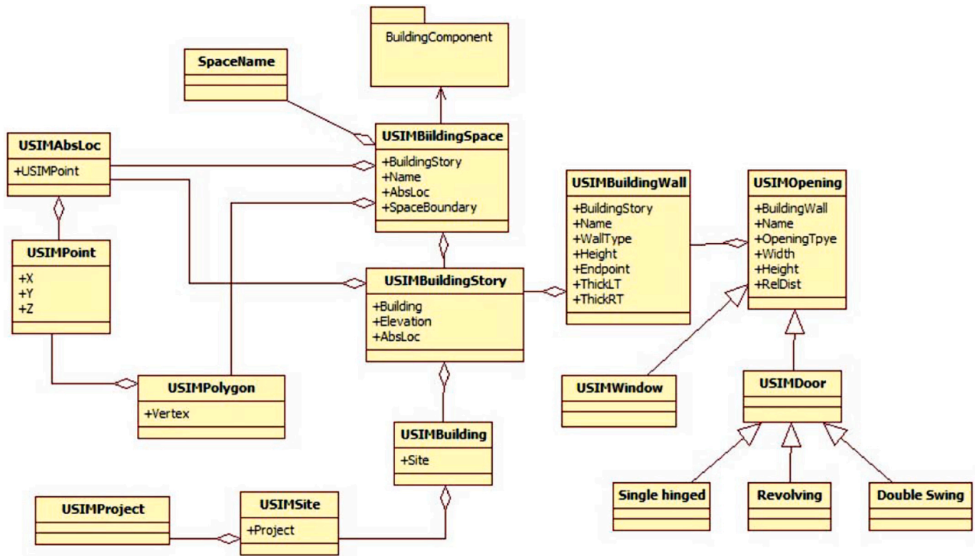
Fig. 13. The Ubiquitous Space Information Model ([75]).
