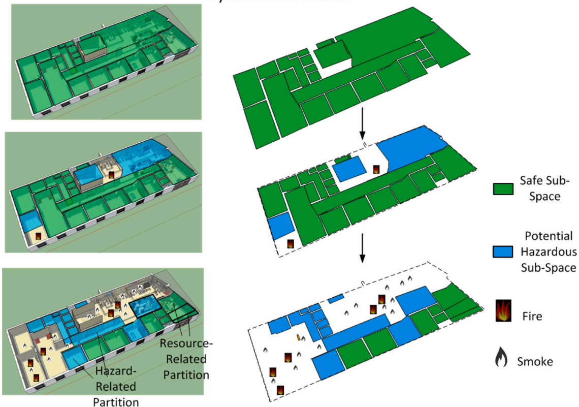
Fig. 16. Extension of fire and smoke in emergencies [36].
