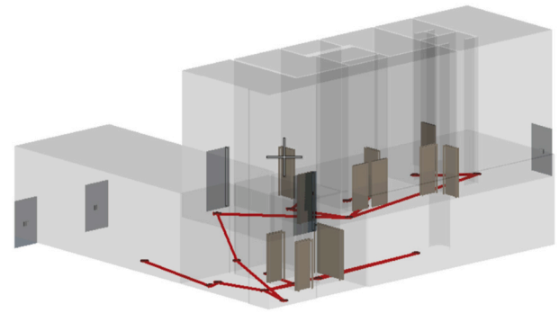
Fig. 6. Topological network derived from IfcSpace instances.
