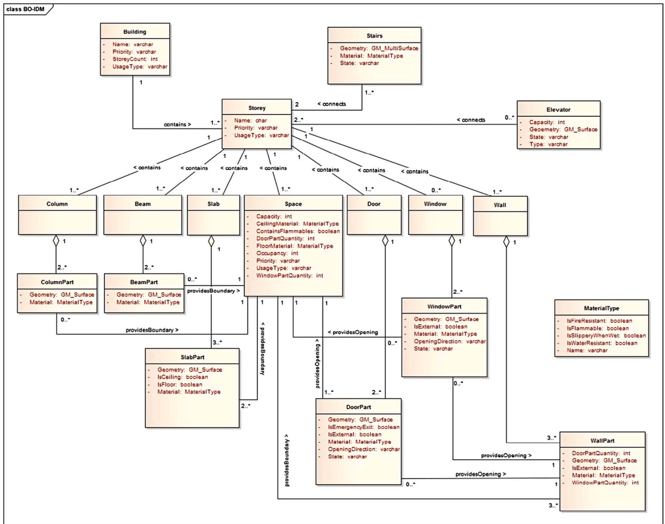
Fig. 14. The BIM Oriented Indoor Data Model, BO-IDM ([7]).
