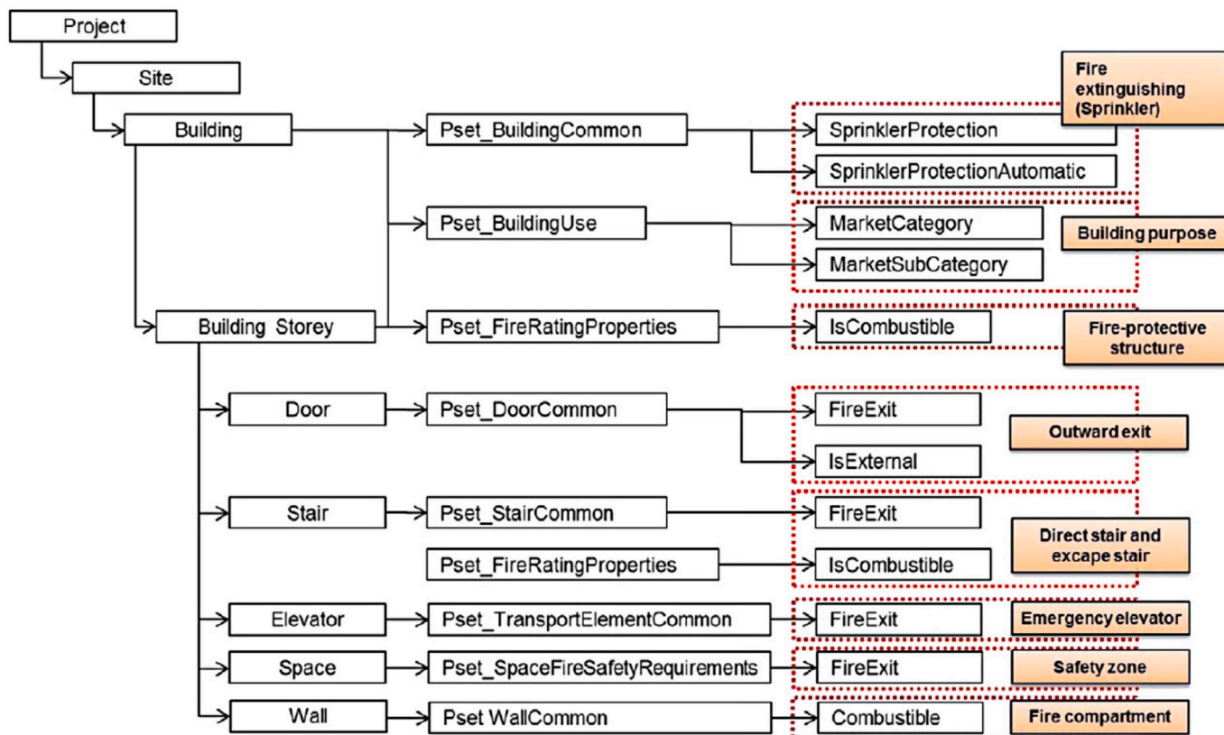
Fig. 17. IFC properties for evacuation regulations ([89]).
