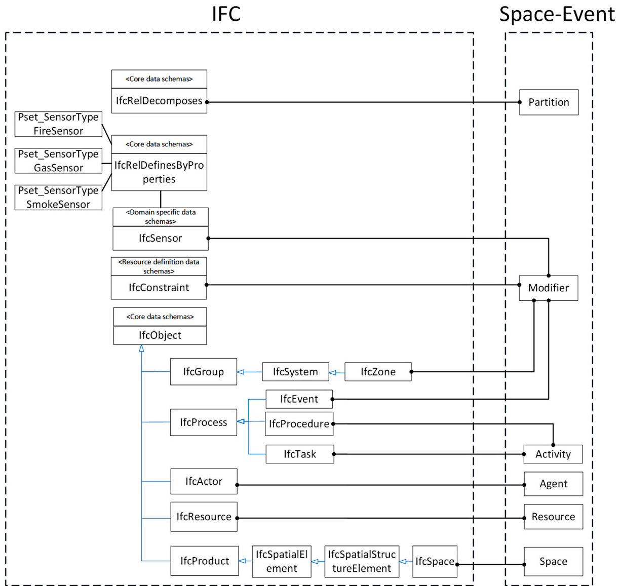
Fig. 21. The relations between the IFC classes and the conceptual framework of space-event.
