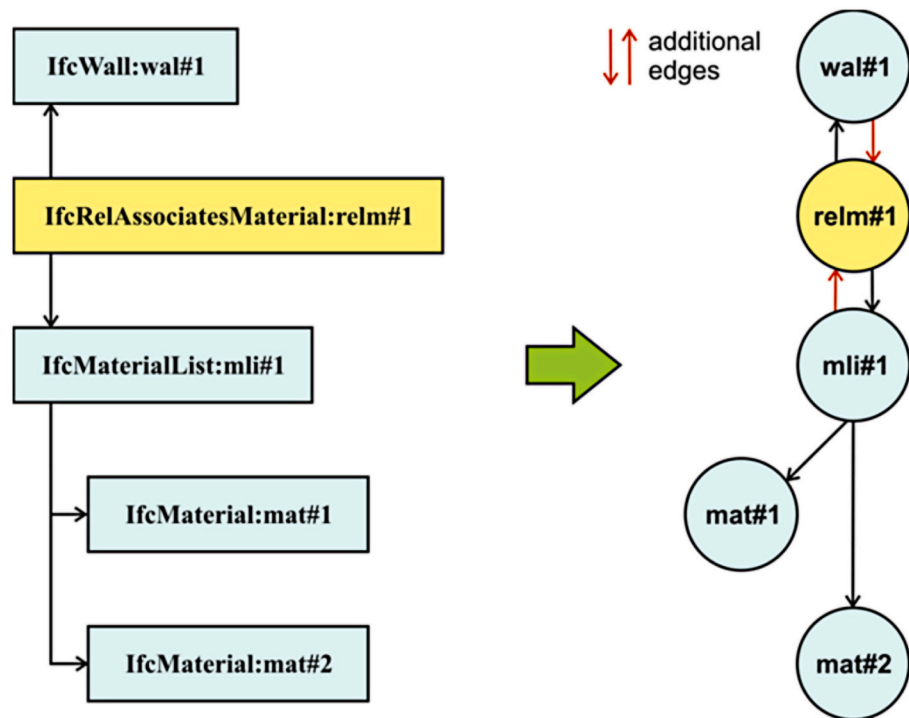
Fig. 7. Transformation from IFC objects to a graph model of building elements ([54]).
