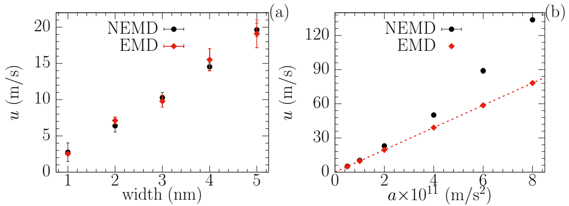
Figure 6. a) Average fluid velocity as a function of the pore width from EMD and NEMD simulations. NEMD data are obtained at an external acceleration 1 \times 10^{11} \text{ m/s}^2 . b) Average fluid velocity with external acceleration for pore width 3 nm. The dotted straight line is prediction from EMD. The error bars show the standard error.
