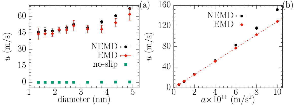
Figure 4. a) Average fluid velocity as a function of the nanotube diameter from EMD and NEMD simulations. NEMD data are obtained at an external acceleration 4 \times 10^{11} m/s 2 . The average velocities calculated using Hagen-Poiseuille formalism with no-slip boundary condition are also shown. b) Average fluid velocity with external acceleration for tube diameter 2.72 nm. The dotted straight line is prediction from EMD. The error bars show the standard error.
