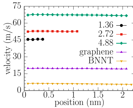
Figure 3. Velocity profiles of water at various positions from NEMD simulation for 1.36, 2.72 and 4.88 nm diameter CNTs, a BNNT of 4.98 nm diameter and 5 nm graphene slit pore. NEMD data are obtained at an external acceleration of 4 \times 10^{11} \text{ m/s}^2 for CNTs and at 1 \times 10^{11} \text{ m/s}^2 for graphene channels.
