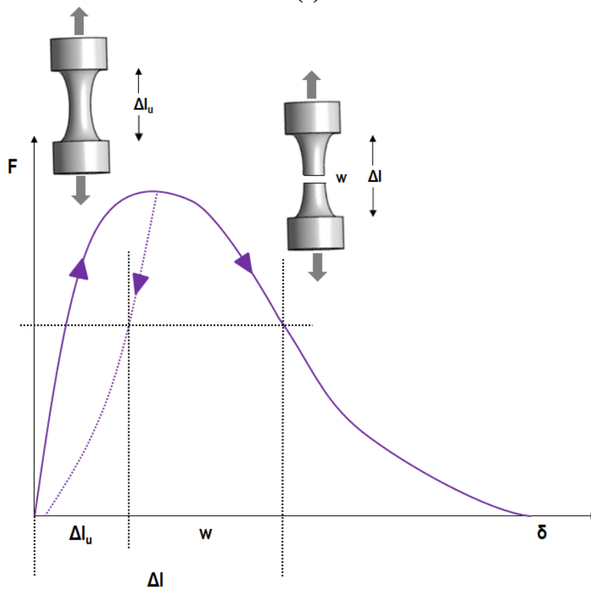
FIGURE 2 Direct tensile testing configuration: (a) specimen fixed in the clamping system after testing, and (b) schematic of uniaxial specimen response in tension
