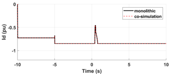
Fig. 5.d: The reference current ( I_d ) of the WT
