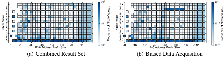
Fig. 3. Probability mass function for each 4bit position in obtained datasets following Foremski et al. [8]. Figure 3(a) visualizes our combined dataset, with 5,766,133 unique IPv6 addresses. Figure 3(b) depicts an artifact from a measurement error in an earlier study.
