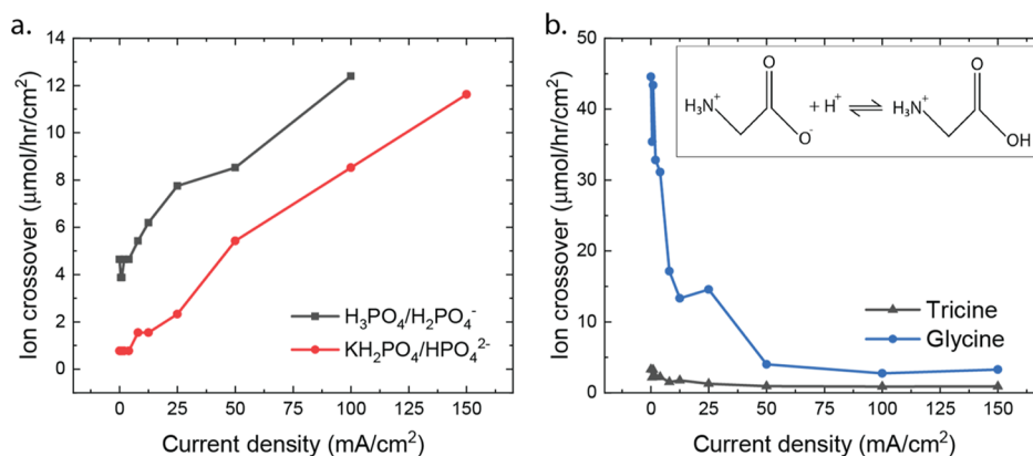
Figure 4. Absolute ion crossover of the (a) phosphate buffers at pK a 2 (black) and pK a 7 (red), which illustrate the dependence of valence for ion crossover and (b) glycine and tricine buffers with cationic species, with the equilibrium reaction of glycine under acidic conditions in the inset. The tricine structure has the same backbone as glycine, with a tris(hydroxymethyl)methyl group attached.
