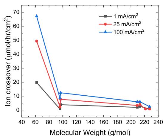
Figure 5. Ion crossover of catholytic anions as a function of molecular weight. Glycine and tricine are excluded because of their zwitterionic form, and no anion crossover of KHCO 3 is measured. Figure S2b represents the same data without boric acid ( M w 61.8 g mol -1 ), which still shows a decreasing trend.
