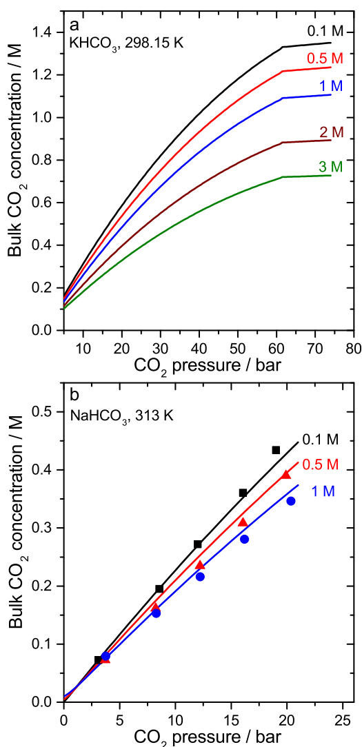
Figure 2. Solubility, concentration of \text{CO}_2 in potassium bicarbonate electrolyte as a function of the pressure, up to 73 bar for several concentrations of potassium bicarbonate at 298.15 K (a) and sodium bicarbonate at 313 K (b). The model is the curves, and the data points in (b) from Xiaoying et al. 78 The curves are produced by following Duan et al. 68 and modeling the bicarbonate concentration as \text{Cl}^- since they have similar salting out effects. 70
