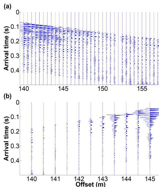
FIGURE 13 Field S-wave reflection data after surface-wave and free-surface multiple suppressions: (a) common-source gather and (b) common-mid-point gather.
