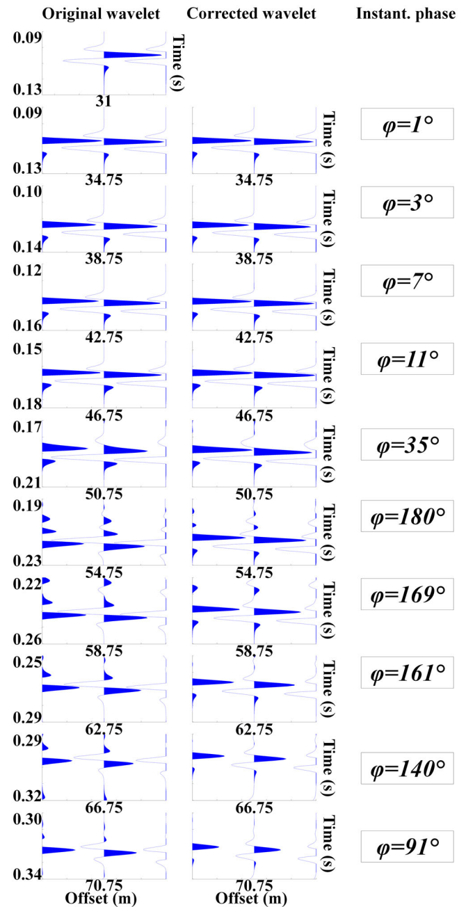
FIGURE 5 Same as in Figure 3, but for the traces shown in Figure 2c.
