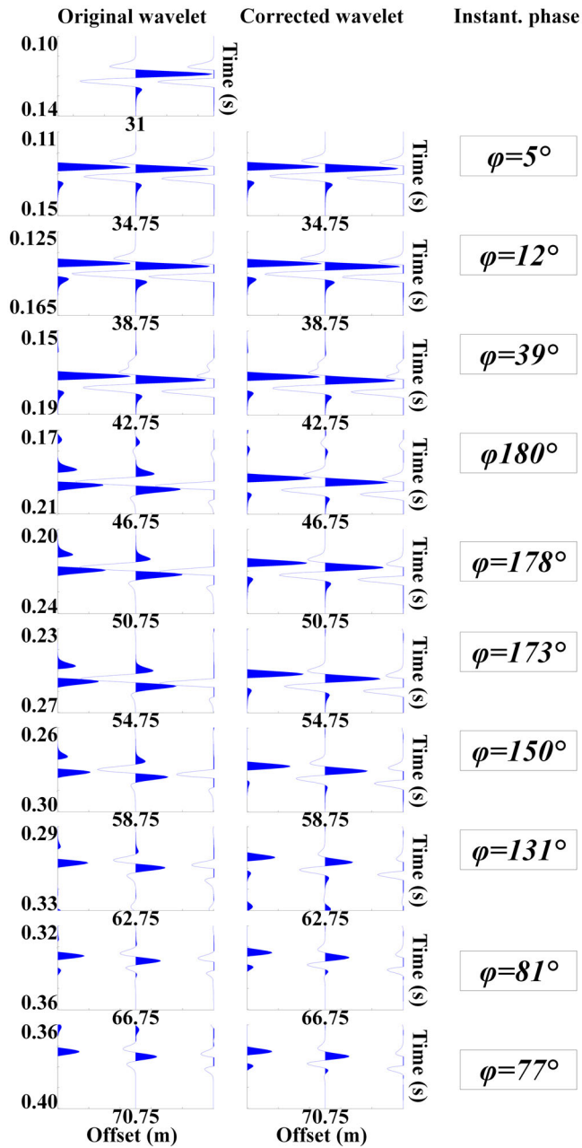
FIGURE 4 Same as in Figure 3, but for the traces shown in Figure 2b.
