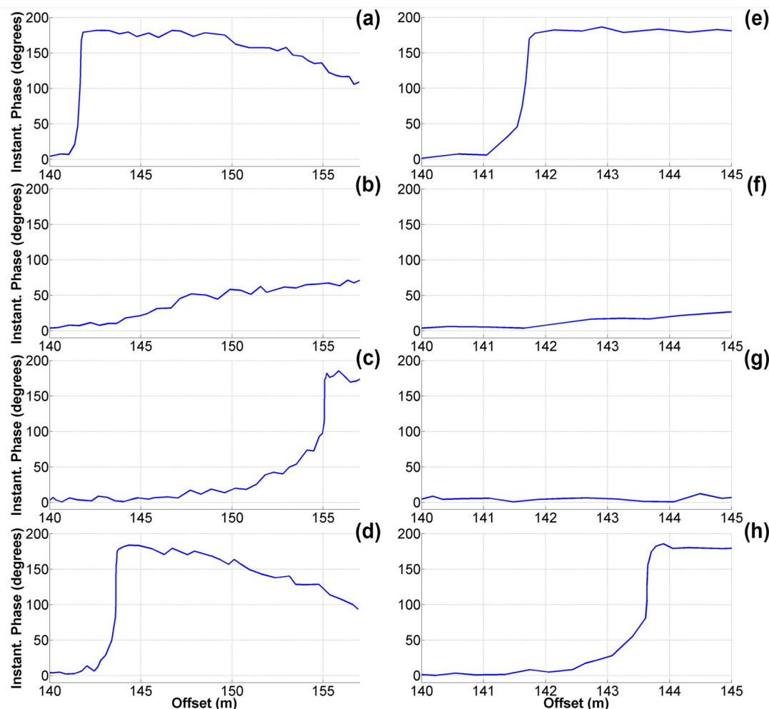
FIGURE 14 Variation of the instantaneous phase with the offset in the field common-source gather for (a) the first, (b) the second, (c) the third and (d) the fourth reflection event. Variation of the instantaneous phase with the offset in the common-mid-point (CMP) gather for (e) the first, (f) the second, (g) the third and (h) the fourth reflection event.
