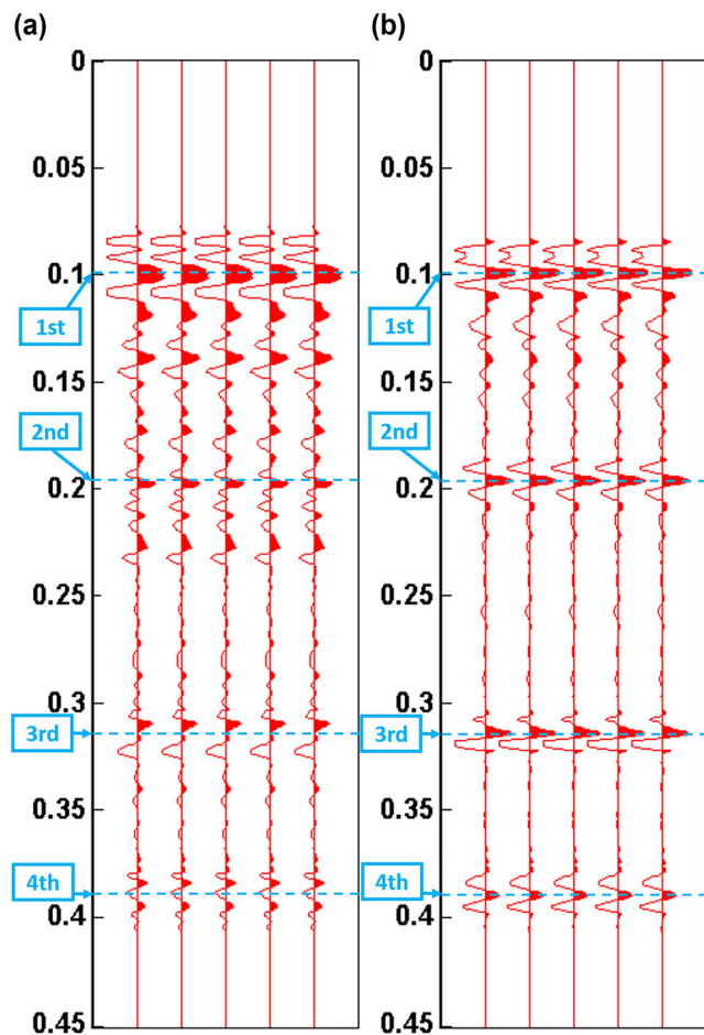
FIGURE 15 Stacked common-mid-point (CMP) sections from near-surface seismic field data: (a) without and (b) with correction for the phase rotation using the proposed approach. The reflection events are marked by the blue dashed lines.
