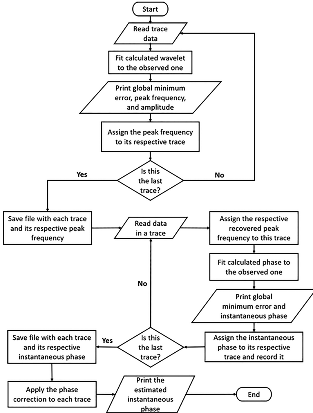
FIGURE 1 Flow chart of the proposed algorithm.
