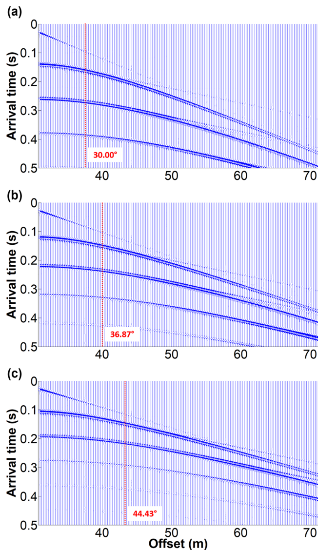
FIGURE 2 Simulated common-source gathers for the three two-layered models used in our tests. The primary reflection for the three models is characterized by a critical angle (CA) at (a) 30.00°, (b) 36.87° and (c) 44.43°, indicated by red dotted line.
