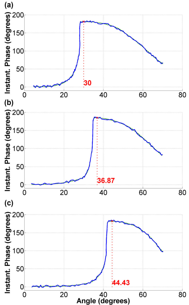
FIGURE 7 Variation of the instantaneous phase as a function of the incidence angle for noisy (signal-to-noise ratio [SNR] = 2, bold blue line) data for the primary reflection event corresponding to (a) Figure 6a, (b) Figure 6b and (c) Figure 6c. The correct critical angle (CA) value is indicated in red for comparison. Moreover, for comparison, the dashed green lines show the results for noise-free data.
