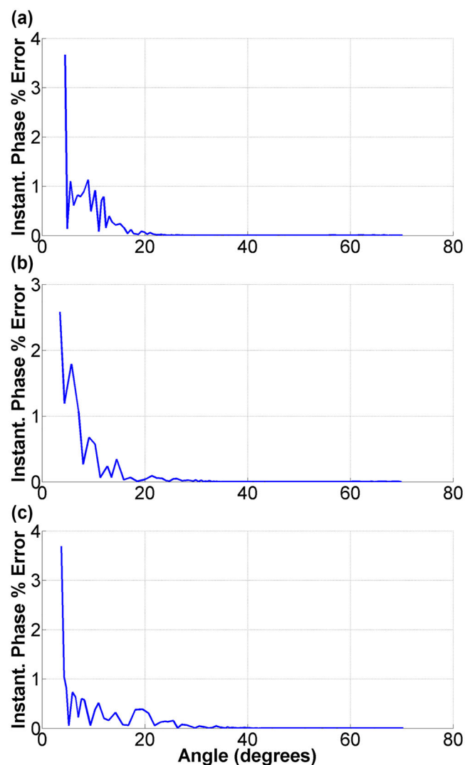
FIGURE 8 Variation of the normalized instantaneous-phase difference {between noise-free and noisy [signal-to-noise ratio (SNR) = 2] data} with the incidence angle for the primary reflection event shown in (a) Figure 6a, (b) Figure 6b and (c) Figure 6c.
