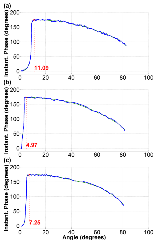
FIGURE 12 Same as in Figure 10, but for the SP reflection event.
