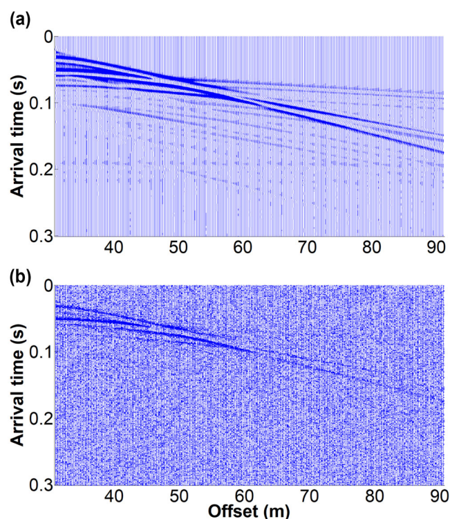
FIGURE 9 Simulated common-source gather using a pressure source on a four-layered elastic model, showing both P- and S-wave reflection events in the case (a) without noise and (b) with noise (signal-to-noise ratio [SNR] = 2) as recorded on the vertical component of a particle-velocity sensor.
