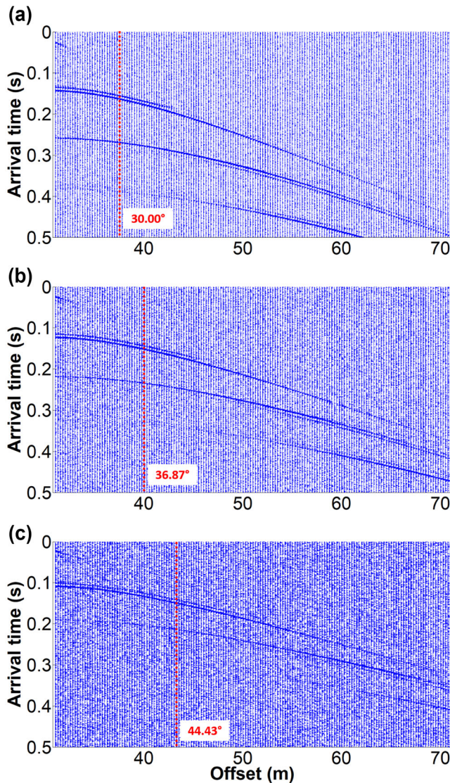
FIGURE 6 Simulated common-source gathers for the three two-layered models, with signal-to-noise ratio (SNR) = 2, used in our tests. The primary reflection for each gather is characterized by a critical angle (CA) at (a) 30.00^\circ , (b) 36.87^\circ and (c) 44.43^\circ , indicated in red.
