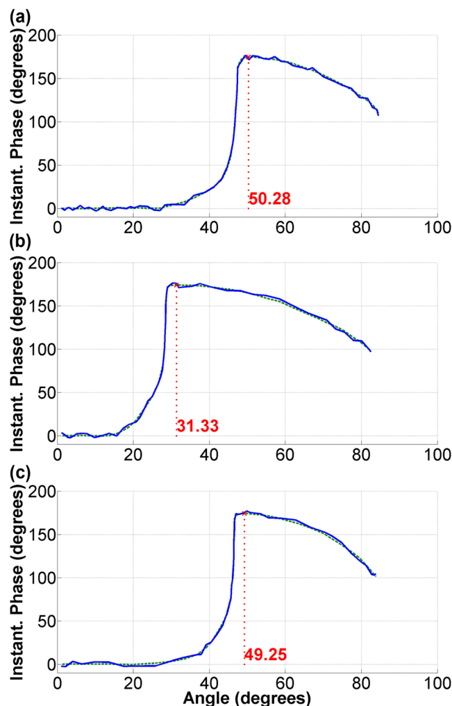
FIGURE 11 Same as in Figure 10, but for the SS reflection event.
