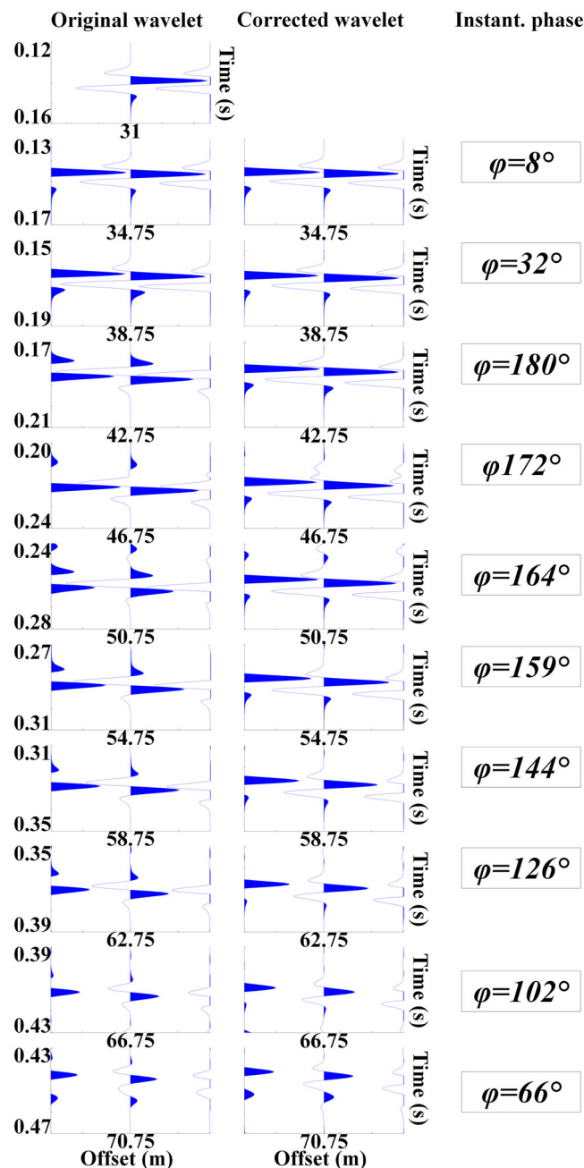
FIGURE 3 Original wavelets from the traces shown in Figure 2A (first column), the corrected wavelets (second column) and the phase shift in degree relative to the first recorded wavelet (third column) for the chosen reflection event.
