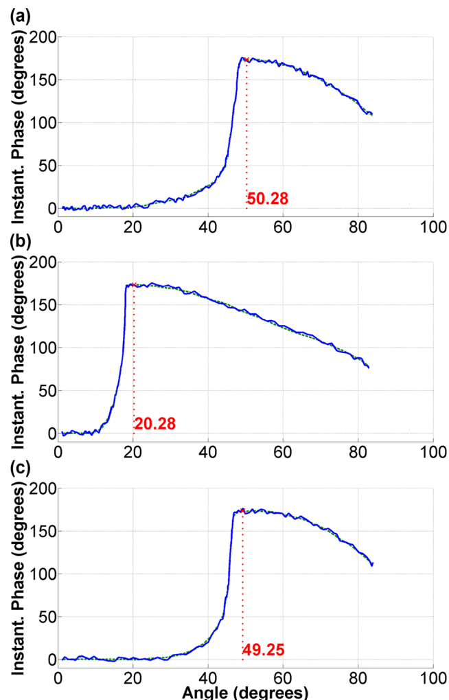
FIGURE 10 Variation of the instantaneous phase with the incident angle for data without noise (dashed green line) and with noise having signal-to-noise ratio (SNR) = 2 (bold blue line), for the PP reflection event in (a) the first layer, (b) the second layer and (c) the third layer. The exact critical angle (CA) is indicated in red, for comparison.
