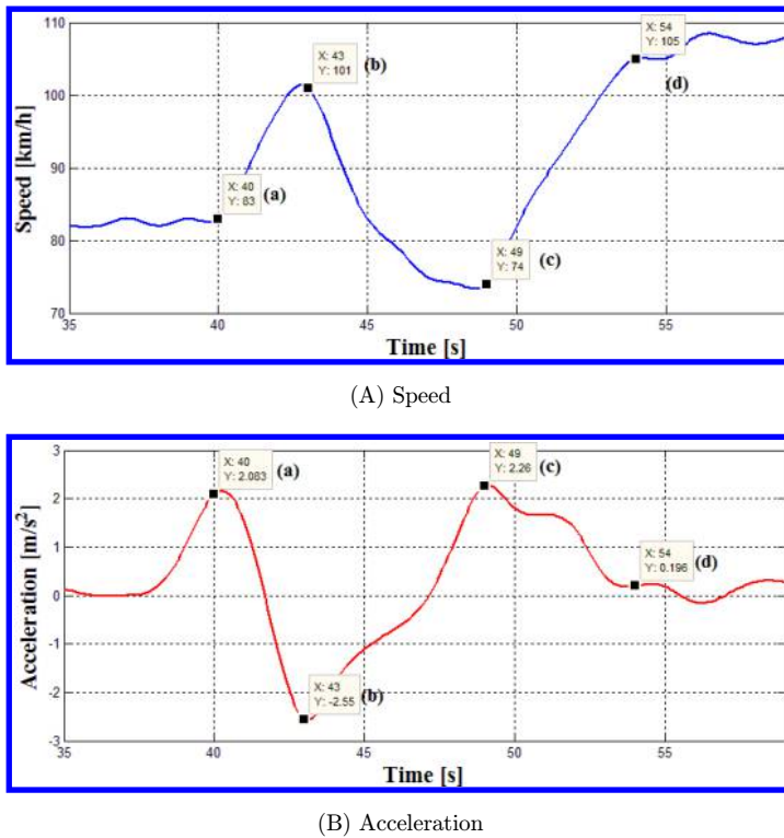
Fig. 4. Time domain plot for speed and acceleration of high-risk driving events.
