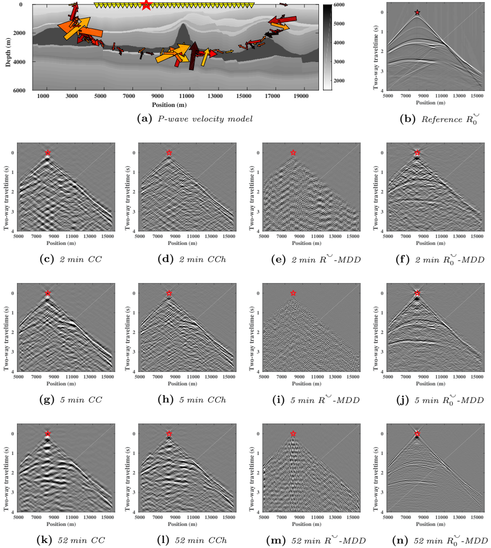
Figure 3.6: Results of different ANSI methods with acoustic ambient noise. (a) P-wave velocity model, with dipole noise sources with random spectrum, random orientation and irregular occurrence. (b) Directly modelled reflection response for an active source at x_0 = 7950 m (the red open star in (a)). (c), (d), (e) and (f) Retrieved virtual common-source gather at the same location using 2 minutes of noise, using crosscorrelation (CC) (c), crosscoherence (CCh) (d), R_0^{\sim} -MDD (e) and R_0^{\sim} -MDD (f). (g), (h), (i) and (j) Same as in (c), (d), (e) and (f), after 5 minutes of noise. (k), (l), (m) and (n) Retrieved results after 52 minutes of noise.
