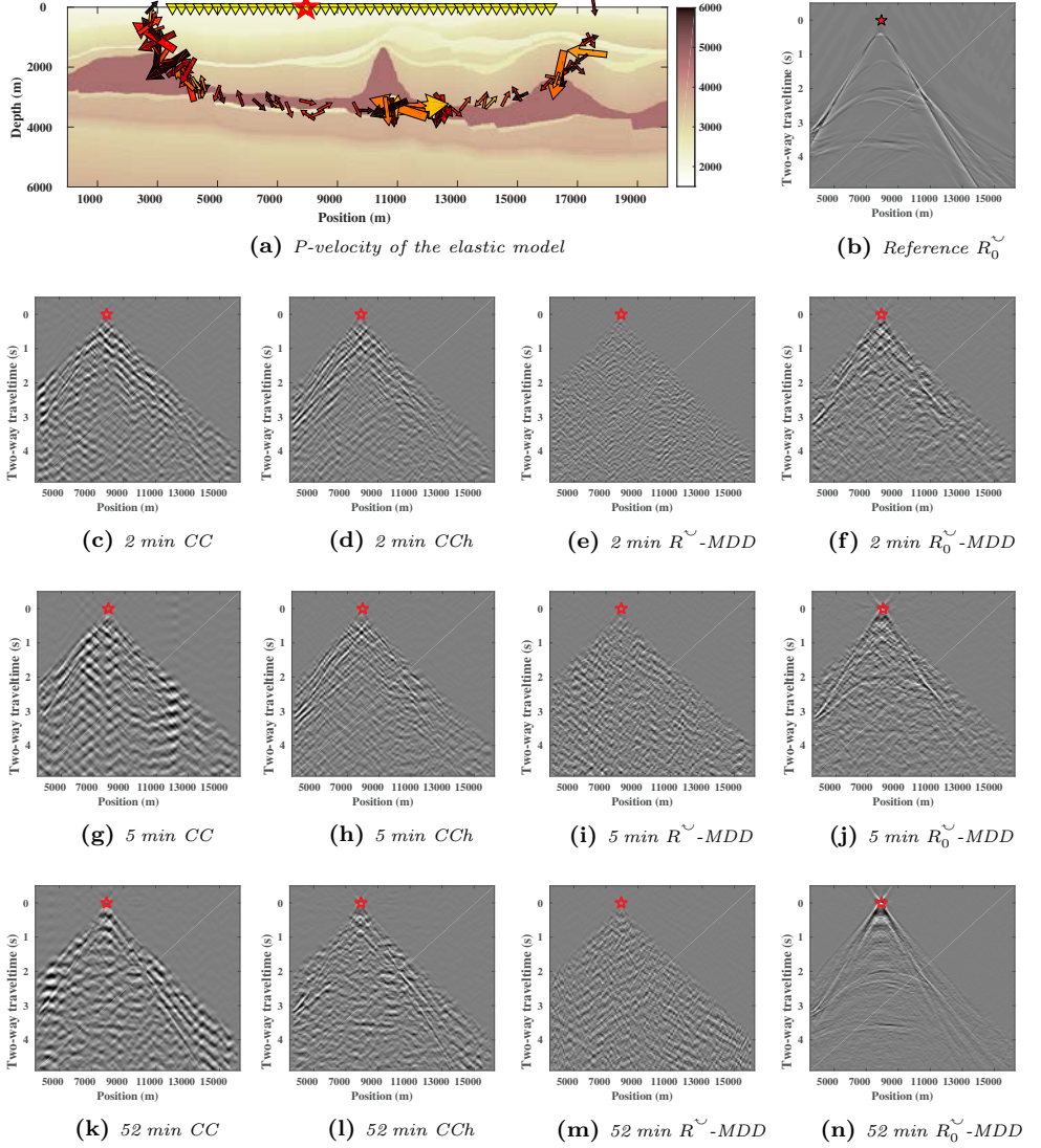
Figure 3.10: Same as in 3.9 for R_0^{\Psi, \Psi} .
