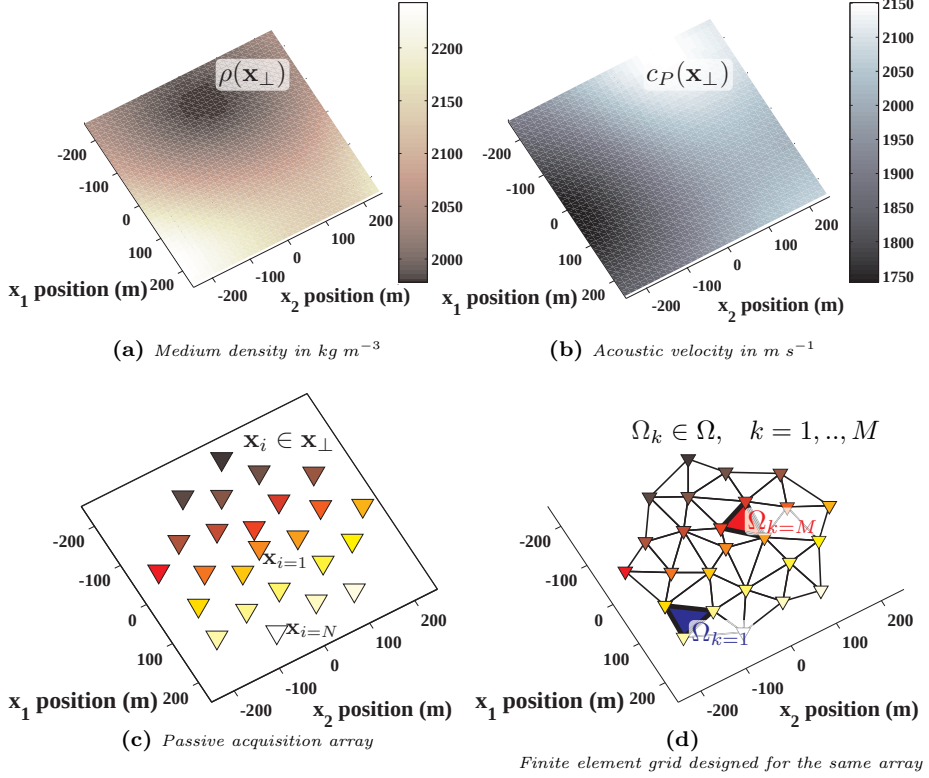
Figure II.1: Example of laterally variant near-surface parameters and a passive acquisition array with irregular grid design. (a) and (b) Mass-density and acoustic velocity maps at a surface of constant depth, respectively. (c) Passive acquisition array with 25 receivers distributed over the same depth level. (d) Finite element grid obtained from the given acquisition array. Elements are identified as \Omega_k and the assembly of the finite elements provides the global matrix operator that approximates the Helmholtz operator. Ill-conceived elements along the edges of the array have been eliminated.
