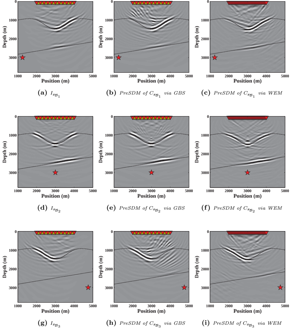
Figure 4.6: (a),(d) and (g) Partial image results I_{x_B} obtained from sources x_{B_1} , x_{B_2} and x_{B_3} , following scenarios in figures 4.3a, 4.3b and 4.3c. (b),(e) and (h) Same as in (a), (d) and (g) using isotropic migration via Gaussian Beam summation method (GBS) on conventional passive interferometry imaging. (c),(f) and (i) Same as in (b), (e) and (h) using one-way wavefield pre-stack depth migration (WEM) on conventional passive interferometry imaging.
