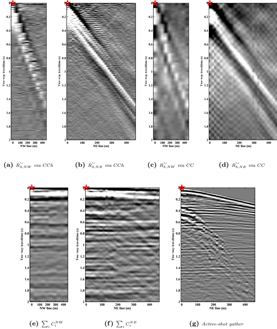
Figure 2.9: Retrieved V_3 -component common-source panels for virtual source at x_0 = 0 m for the NE line and x_0 = 0 m for the NW line. (a) Cross-coherence result (CCh) for the NW line. (b) Cross-coherence result (CCh) for the NE line. (c) Cross-correlation result (CC) using all panels for the NW line. (d) Cross-correlation (CC) result using all panels for the NE line. (e) Same result as in (c) after discrimination and discard of panels with dominant surface waves. (f) Same as in (e) for the NE line. (g) Reference response for an active source located at the surface above the virtual-source location.
