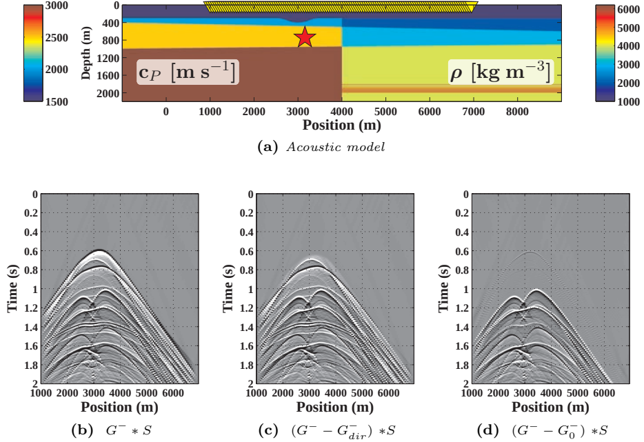
Figure 3.2: Upgoing wavefield and the differences in approximating the free-surface interaction wavefield. (a) Acoustic model represented by its velocity c_P (left) and density \rho (right), with a passive source (red star) and an array of receivers at 10 m depth (yellow triangles). (b) Upgoing wavefield \hat{G} with transient source signal \hat{S} . (c) Free-surface interaction obtained from subtracting the direct wavefield from the upgoing wavefield only, as expressed in equation 3.4 ( G_0^- \approx G_{dir}^- ). (d), same as in (b), using the correct reference transmission response without free surface multiples G_0^- , as required in equation 3.3. By applying the direct wave subtraction, the events present in (b) but not in (c) are left off for the inversion process to produce spurious events in the retrieved reflection response.
