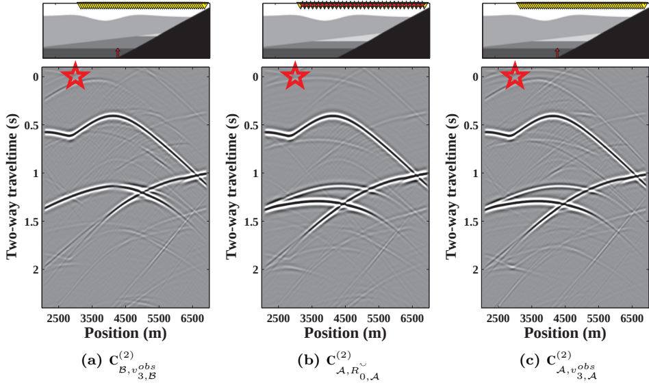
Figure 5.8: (a) Correlation function of the full-field relation C_{B, v_{3,B}^{obs}}^{(2)} at virtual source x_0 = 3000 m, of the monitor state \mathcal{B} . (b) Equivalent correlation function at the same location, virtually generated with the illumination induced from the passive source at state \mathcal{B} , C_{A, R_{0,A}^{v_{3,B}^{obs}}}^{(2)} . (c) Correlation function of the full-field relation 5.25 at the base state \mathcal{A} , C_{A, v_{3,A}^{obs}}^{(2)} .
