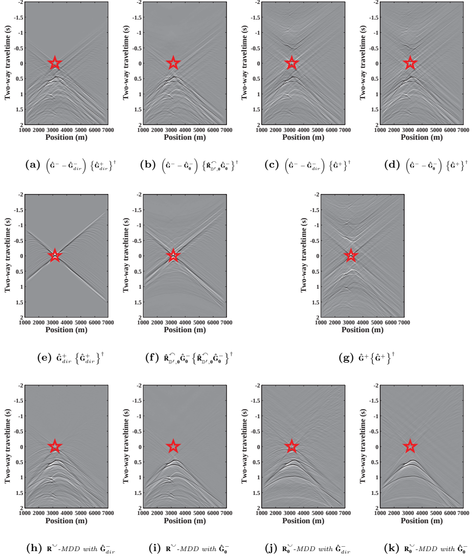
Figure 3.5: Comparison between slices of the different functions in the MDD methods. (a) and (b), R^{\sim} -MDD correlation functions with and without approximation, respectively. (c) and (d), same as in (a) and (b) for R_0^{\sim} -MDD. (e) and (f), the respective R^{\sim} -MDD point-spread functions with the direct wave approximation and the exact approach. (g), R_0^{\sim} -MDD point-spread function. (h) and (i), R^{\sim} -MDD result with the direct wave approximation and without, respectively. (j) and (k), same as in (h) and (i) for R_0^{\sim} -MDD.
