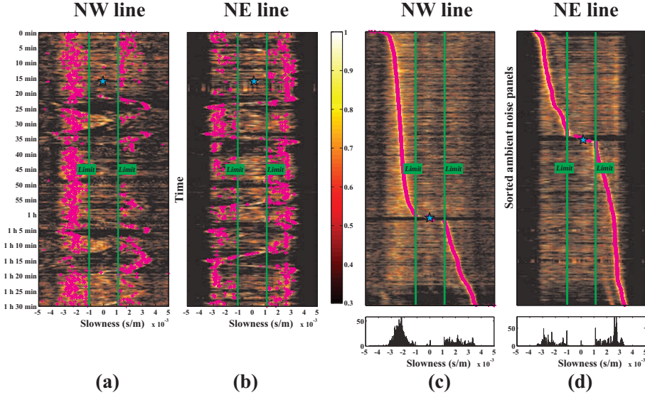
Figure 2.7: Illumination diagnosis with 90 minutes of the total noise record from Figure 2.6. (a) Illumination record for the NW line at position x_0 = 0 m. Ray-parameter p_i^{x_0} is highlighted with a cyan star (dominating body waves) or a magenta dot (dominating surface waves), (b) Illumination record for the NE line at position x_0 = 0 m. (c) Illumination diagnosis for all correlated panels in (a), with the dominant ray-parameters p_i^{NW, x_0} highlighted; Diagram below shows the histogram of p_i^{NW, x_0} . (d) Illumination diagnosis for all correlated panels in (b). Diagram below shows the histogram of p_i^{NE, x_0} .
