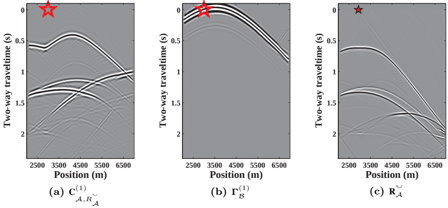
Figure 5.4: (a) Correlation function due to the ballistic relation 5.22 ( C_{A,R_A}^{(1)} ) at virtual source x_0 = 3000 m, of the reference state A with the illumination induced from the passive source in state B . (b) Point-spread function \Gamma_B^{(1)} at the same location due to the passive source recording v_{3,B}^{obs} in state B (see Figures 5.3b and 5.3d). (c) Reflection response R_A^\sim at x_0 = 3000 m in state A , with free-surface interaction.
