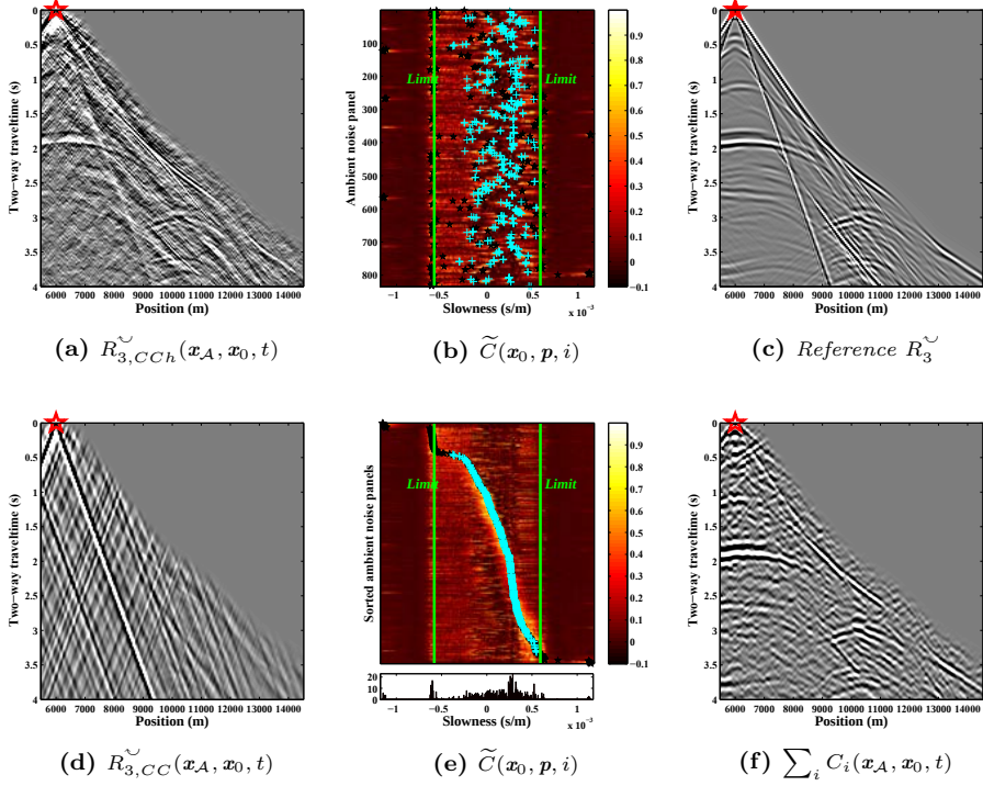
Figure 2.3: Illumination diagnosis for random noise sources in the model shown in Figure 2.2a. (a) Retrieved virtual common-source panel for a virtual-source position x_0 = 6000 m obtained using SI by crosscoherence (CCh). (b) Illumination record, constructed using 834 noise panels of 10 s length, with 5 s of record overlap. (c) Directly modelled common-source panel for an actual source at the virtual-source position. (d) Retrieved common-source panel with SI by cross-correlation (CC), obtained using all correlated panels. (e) Illumination diagnosis, with body-wave dominated panels highlighted in cyan at their characteristic ray-parameter p_i^{x_0} ; Diagram beneath shows the histogram of p_i^{x_0} . (f) Same result as in (d) after discrimination and discard of panels with dominant surface waves, e.g. after summation only over the correlated panels with cyan stars, weighted according to the histogram in (e).
