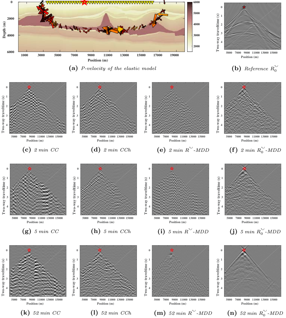
Figure 3.11: Same as in 3.9 for R_0^{\Psi, \Phi} .
