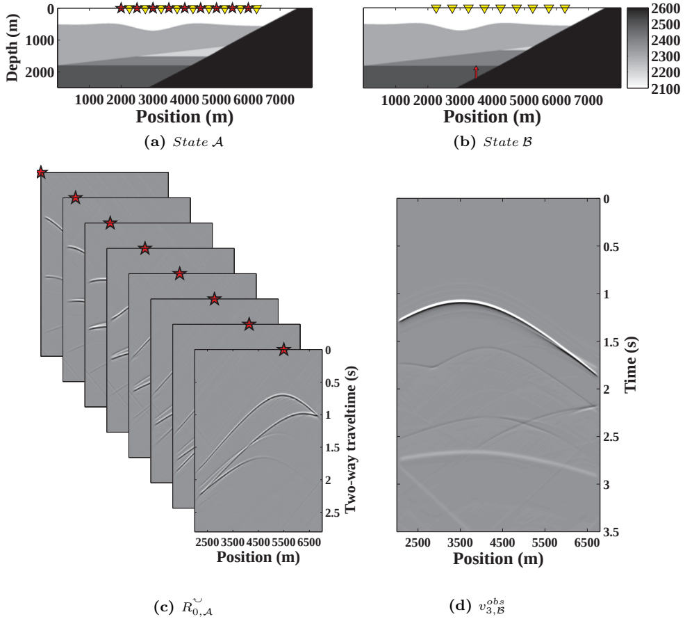
Figure 5.3: Set-up for one of the alternative monitoring schemes: (a) Acoustic velocity model ( \text{m s}^{-1} ) at state \mathcal{A} (base survey): controlled sources and receivers are located at the Earth's surface. (b) Model at state \mathcal{B} (monitor survey) with a single passive source in the subsurface (red star). (c) Reflection response survey at state \mathcal{A} (as displayed in (a)), where the surface-related multiples have been removed ( R_{0,\mathcal{A}}^{\sim} ). (d) Passive source recording v_{3,\mathcal{B}}^{obs} at state \mathcal{B} , as illustrated in (b).
