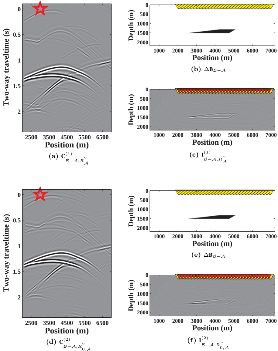
Figure 5.11: (a) Correlation function difference between the monitor and base states using the ballistic relation, C_{B-A, R_{\mathcal{A}}}^{(1)} . This is the difference between figures 5.5a and 5.5b. (b) Medium-property contrast between states \mathcal{A} and \mathcal{B} . (c) Directionally constrained image of the correlation function difference C_{B-A, R_{\mathcal{A}}}^{(1)} , using the same forward wavefield as for the results in figure 5.10. (d) Same as in (a) but using the full-field relation, C_{B-A, R_{0, \mathcal{A}}}^{(2)} . This is the difference between figures 5.7a and 5.7b. (e) Medium-property contrast between states \mathcal{A} and \mathcal{B} . (f) Same as in (c) but using the full-field relation.
