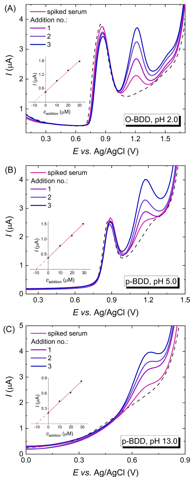
Fig. 7. DP voltammograms recorded in the synthetic serum samples diluted with the corresponding supporting electrolyte (1:4) and spiked with 10 \mu\text{M} NVP, followed by the three standard additions (all 100 \mu\text{L} , 1 mM NVP) on (A) O-BDD (pH 2.0), (B) p-BDD (pH 5.0), and (C) p-BDD (pH 13.0). Dashed lines correspond to the diluted synthetic serum sample without spiked NVP. Insets demonstrate the graphical quantification of NVP using a standard addition method.
