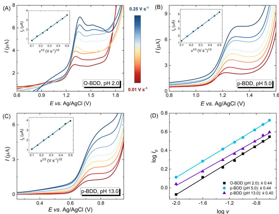
Fig. 3. LS voltammograms of 100 \mu\text{M} NVP for the range of scan rates \nu on (A) O-BDD in 0.04 M BR buffer (pH 2.0), (B) p-BDD in 0.1 M acetic buffer (pH 5.0), and (C) p-BDD in 0.1 M NaOH (pH 13.0). Insets in (A–C) display linear dependence of NVP peak currents ( I_p ) on the square root of the scan rate ( \nu^{1/2} ). (D) Dependences of \log I_p vs. \log \nu along with the slope values acquired from the scan rate studies.
