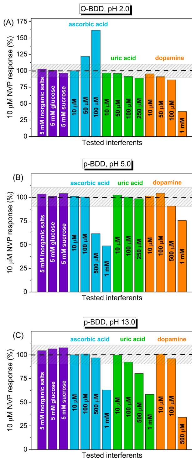
Fig. 6. Relative DP voltammetric response of 10 \mu\text{M} NVP acquired in the presence of several interfering compounds at different concentration levels on (A) O-BDD electrode in 0.04 M BR buffer of pH 2.0, (B) p-BDD electrode in 0.1 M acetic buffer of pH 5.0, and (C) p-BDD electrode in 0.1 M NaOH (pH 13.0). The dashed grey zones indicate the tolerated \pm 10\% alteration in the peak current intensities of NVP signals.
