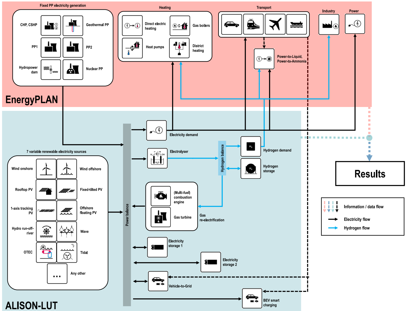
Fig. 5. Schematic overview on the structure of ALISON-LUT and interconnection with EnergyPLAN as the basic modelling platform.
