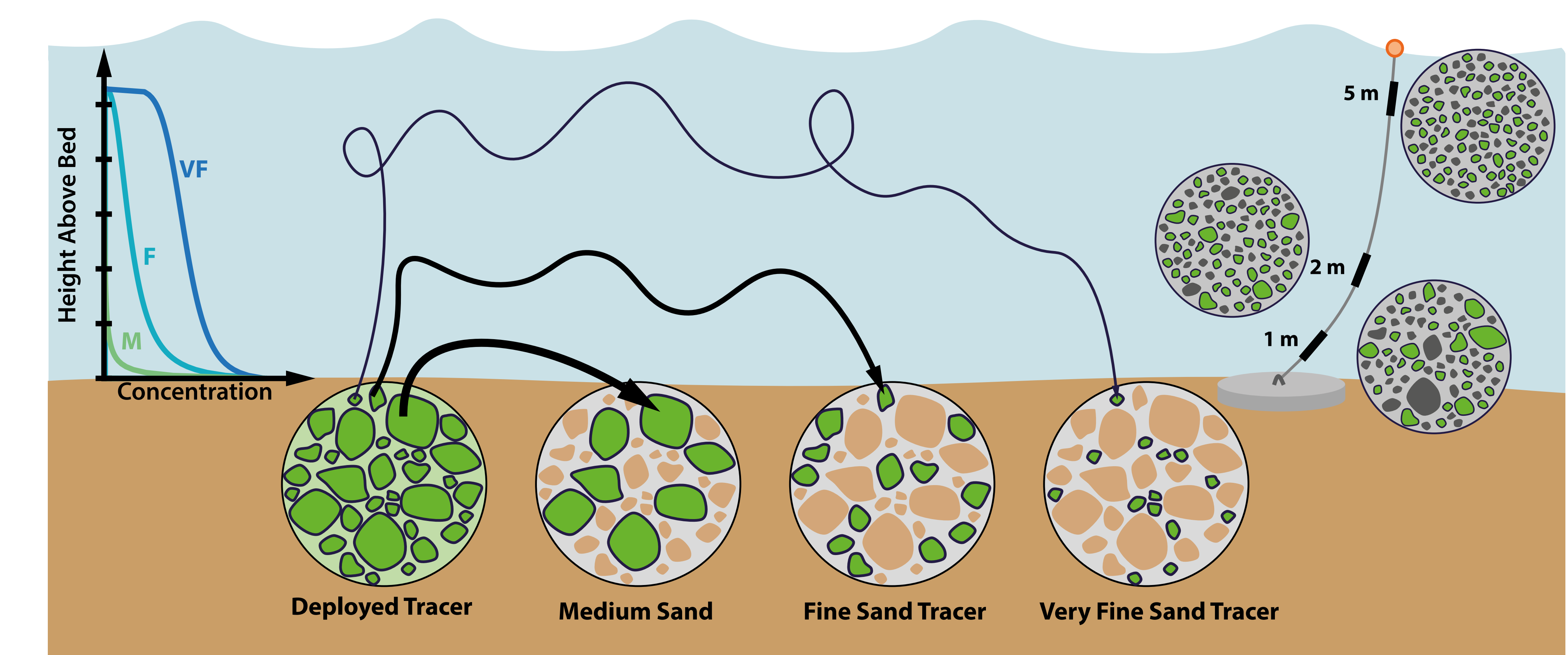
Figure 6. Conceptual diagram indicating dispersal of tracer on the seabed and in the water column. Finer grains are preferentially resuspended and transported further than coarser grains, which travel more often as bedload.
