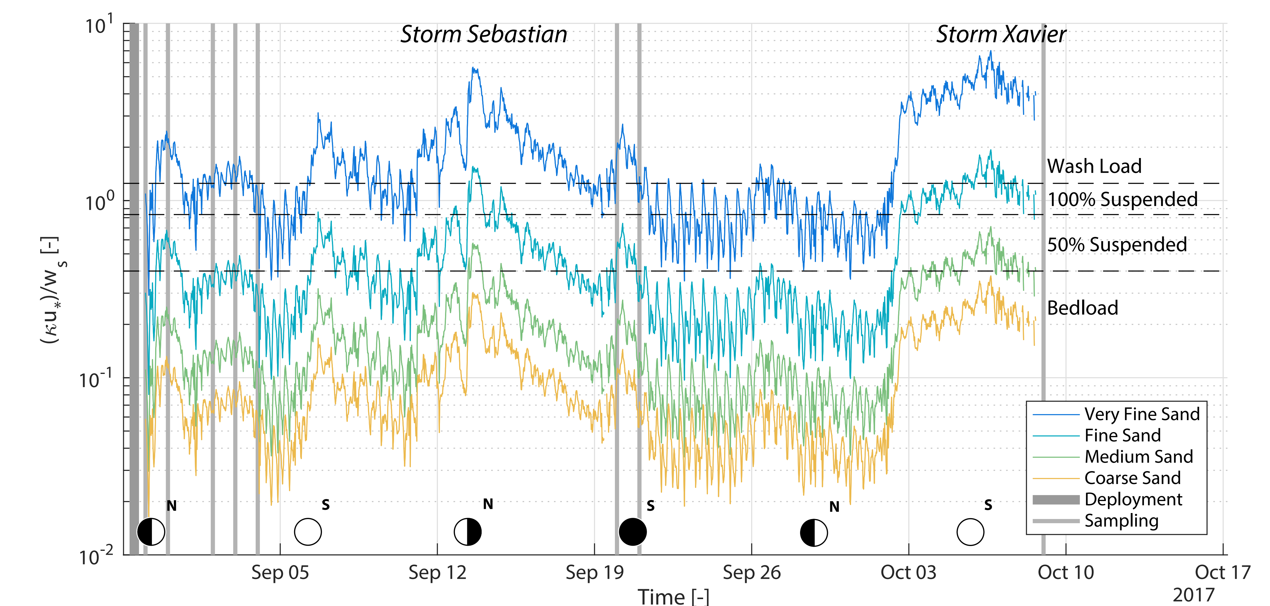
Figure 5. Inverse Rouse number ( \kappa u_s/w_s ) and transport mode for each sediment class. Calculated using the method of Soulsby (1997) from wave and near-bed velocity measurements taken near the tracer source.
