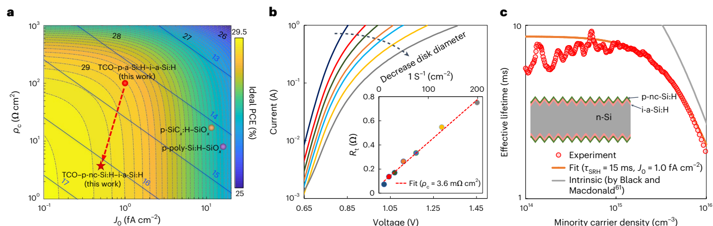
Fig. 4 | Evaluation of the carrier selectivity of HSCs based on a p-nc-Si:H layer.
