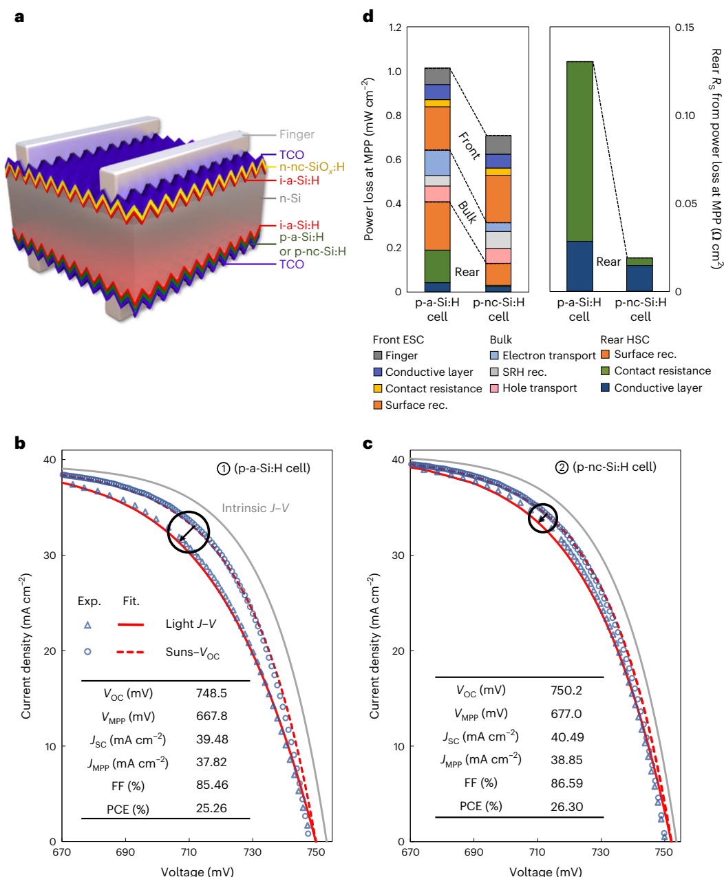
Fig. 2 | Electrical performance of LONGi SHJ solar cells with different designs. a , Diagram of LONGi SHJ solar cells. b, c , Experimental (Exp.) and fitted (Fit.) J - V curves for the p-a-Si:H cell ( b , cell 1 in Fig. 1) and the p-nc-Si:H cell ( c , cell 2 in Fig. 1). The fitted curves are derived from the Quokka2 simulations (Methods). Intrinsic J - V curves are obtained according to the Richter et al. model of intrinsic recombination with photon recycling (photon recycling coefficient of 0.6) 65,71 .
